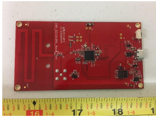
EUT Internal View – Internal antenna version
