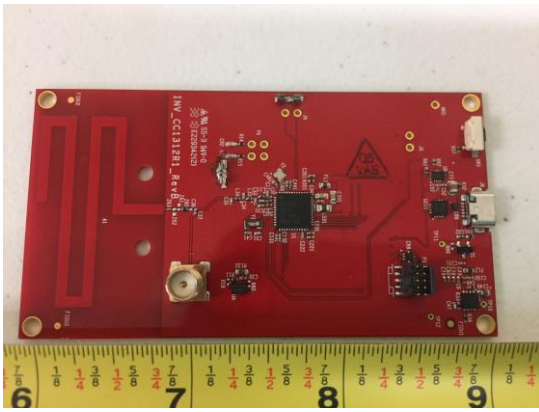
EUT Internal View – External antenna version
