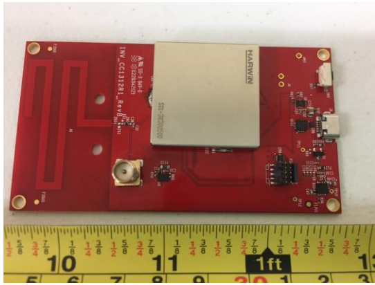
EUT Top View – External antenna version
