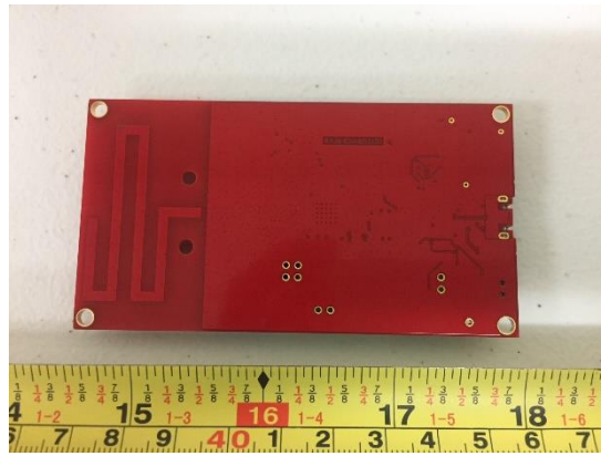
EUT Bottom View – External antenna version
