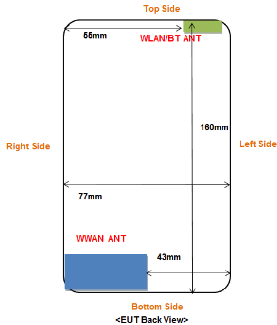
Block Diagram for EUT Antenna Position
