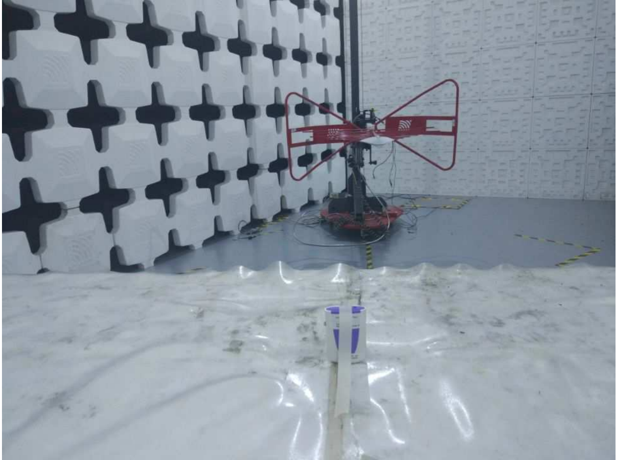
Below 1GHz
