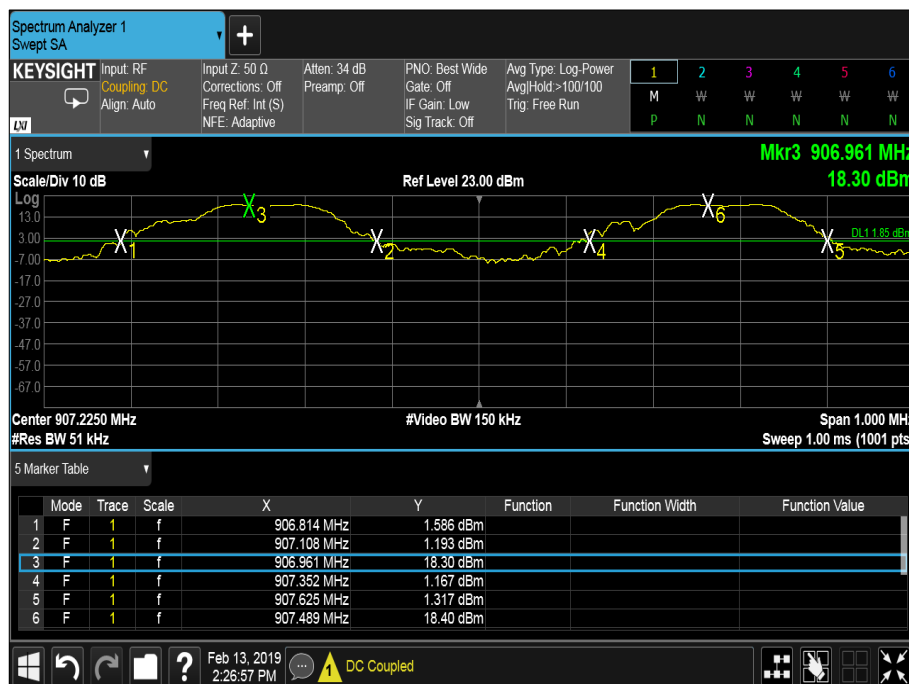
Figure 8, Channel Separation
