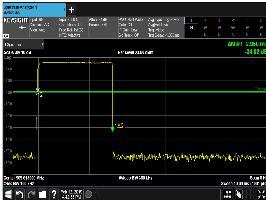
Figure 6 - Dwell Time
