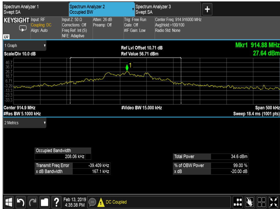
Figure 11 - 914.90 MHz
