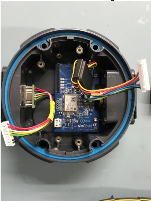
Photo 3: Base of unit showing DGPS PCB
