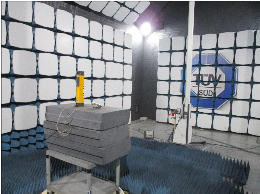
Figure 2 - Test Setup - 1 GHz to 18 GHz
