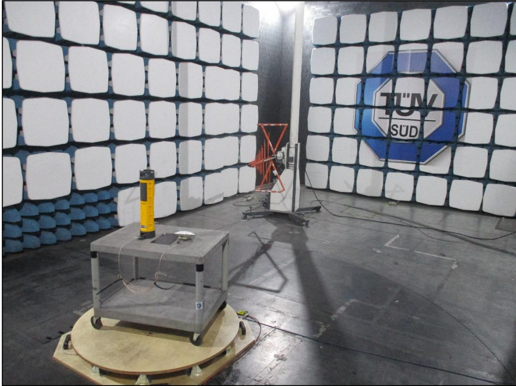
Figure 1 – Test Setup- 30 MHz to 1 GHz
