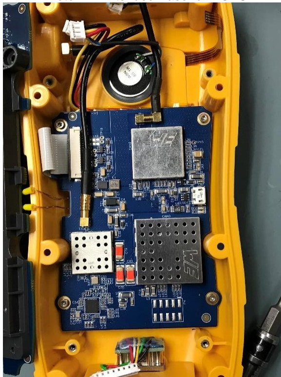
Photo 12: Extended Base for DGPS
