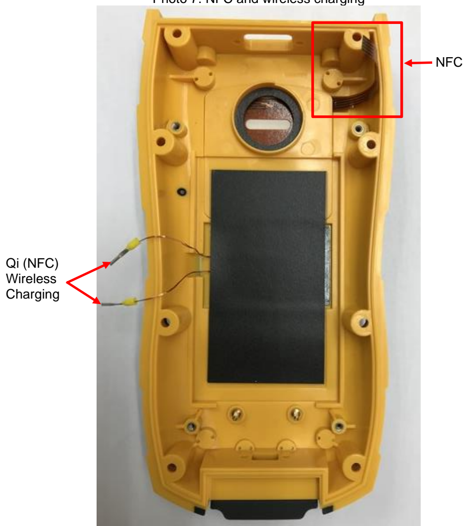
Photo 7: NFC and wireless charging
