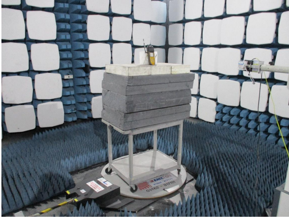
Figure 5 - Test Setup - 18 GHz to 25 GHz
