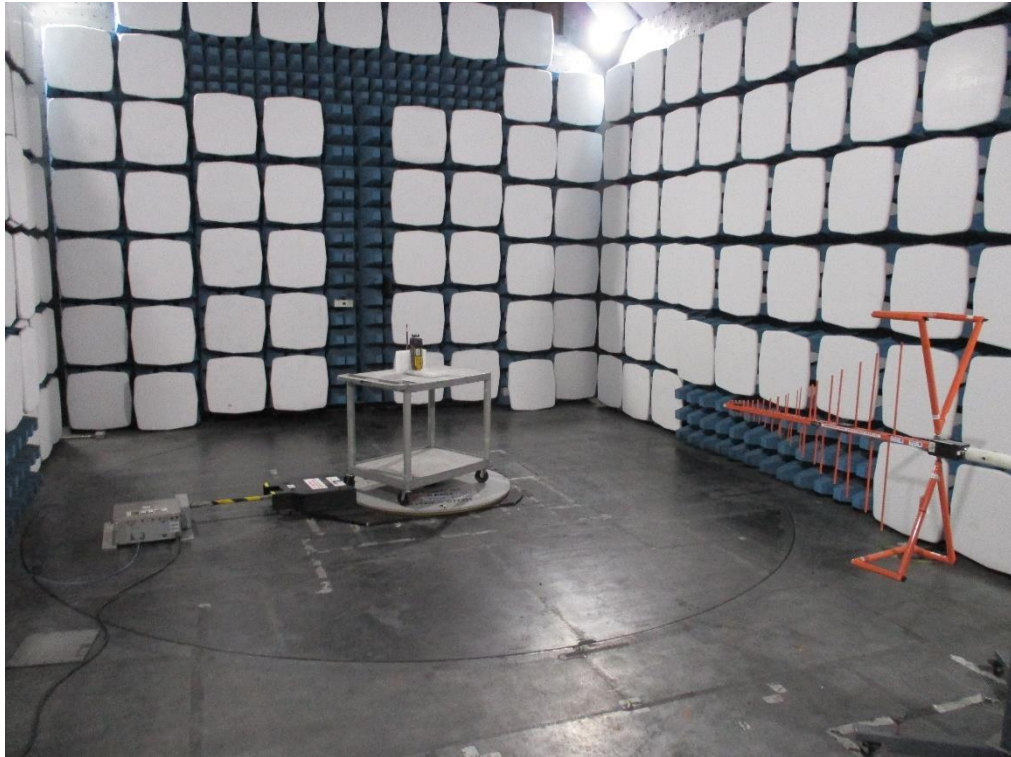
Figure 3 – Test Setup- 30 MHz to 1 GHz, Z Orientation
