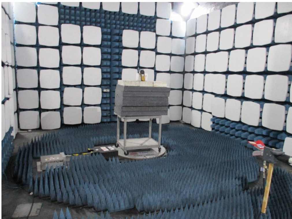
Figure 4 - Test Setup - 1 GHz to 18 GHz
