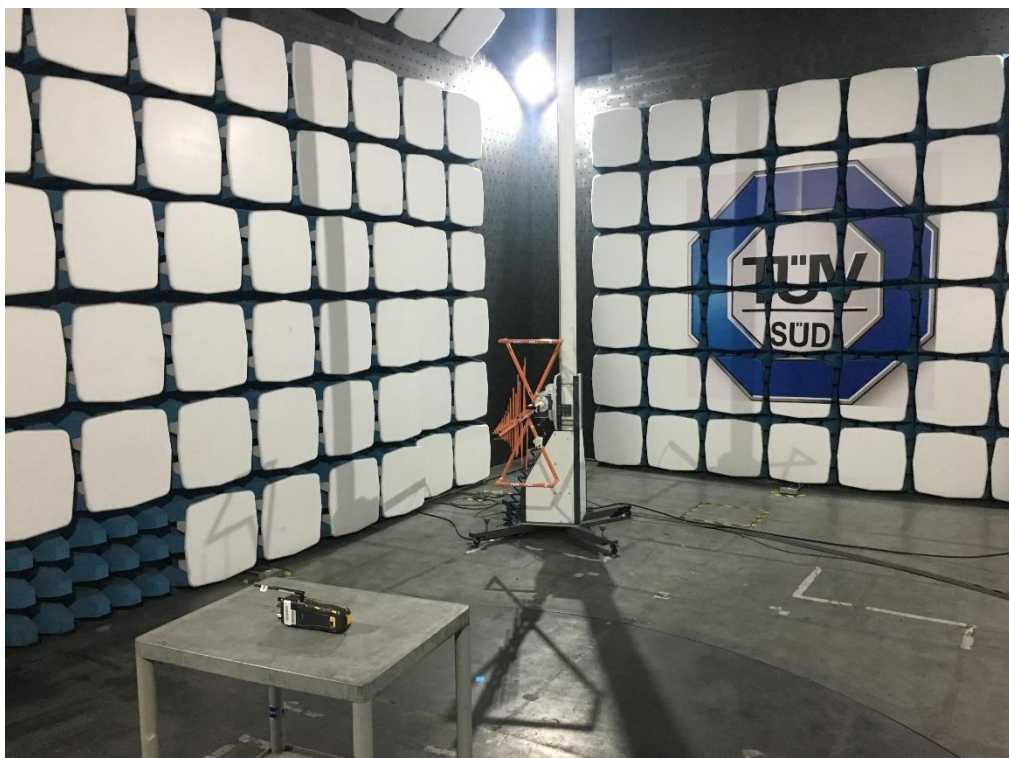
Figure 2 – Test Setup- 30 MHz to 1 GHz, Y Orientation
