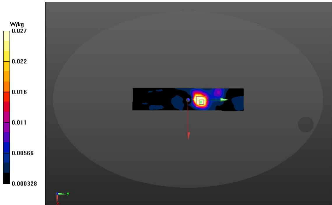
Figure C.3: SAR Body Testing Results for the CE4 Tagger at 2457 MHz - Right - 0mm Separation Distance
