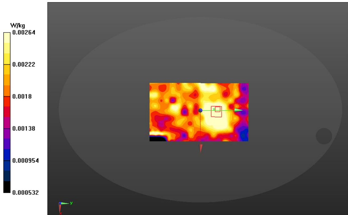
Figure C.4: SAR Body Testing Results for the CE4 Tagger at 2457 MHz - Top - 0mm Separation Distance
