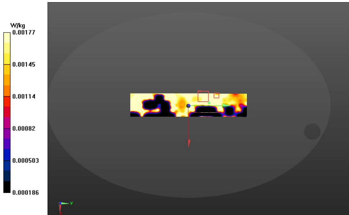
Figure C.5: SAR Body Testing Results for the CE4 Tagger at 2457 MHz - Left - 0mm Separation Distance
