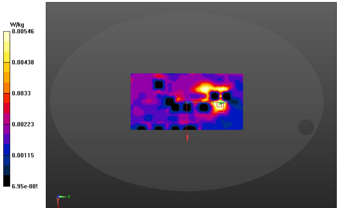
Figure C.2: SAR Body Testing Results for the CE4 Tagger at 2457 MHz - Rear - 0mm Separation Distance
