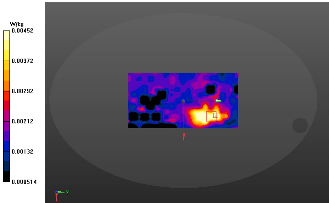
Figure C.1: SAR Body Testing Results for the CE4 Tagger at 2457 MHz - Front - 0mm Separation Distance
