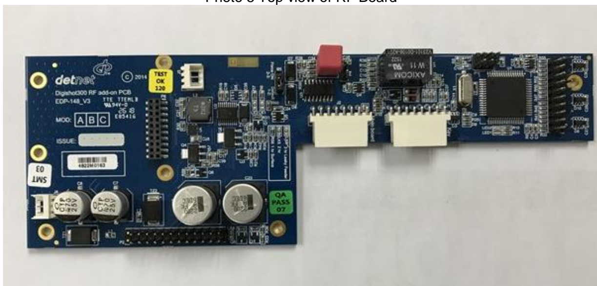
Photo 5 Top view of RF Board
