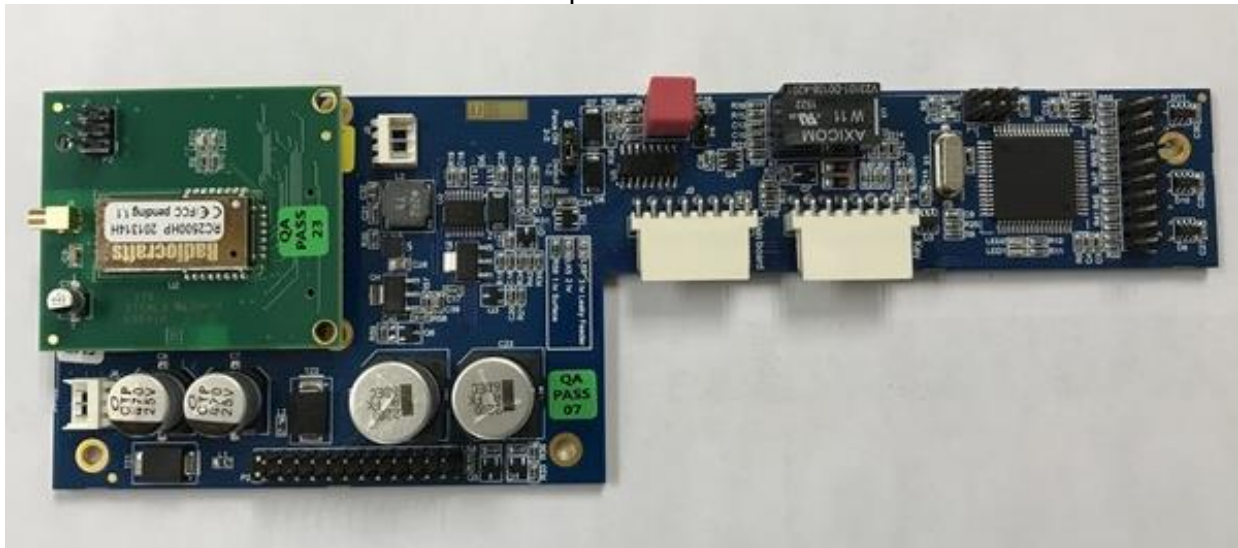
Photo 7 Top view of RF Board
