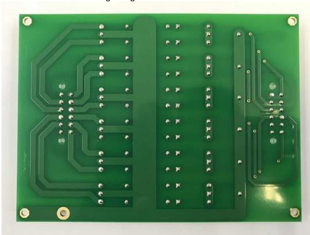
Photo 6: Lightning Protection Board bottom view
