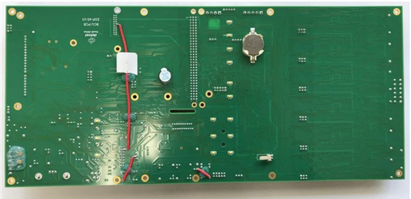
Photo 2: Bottom view
