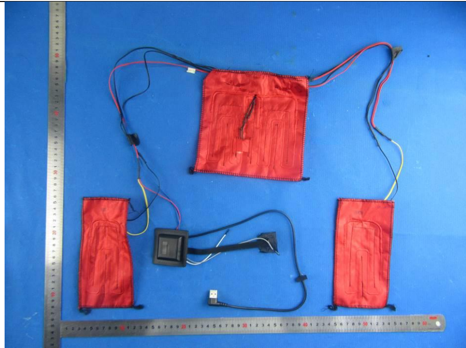
Photo 1 (For model Mercury Intelligent Heated Jacket)
