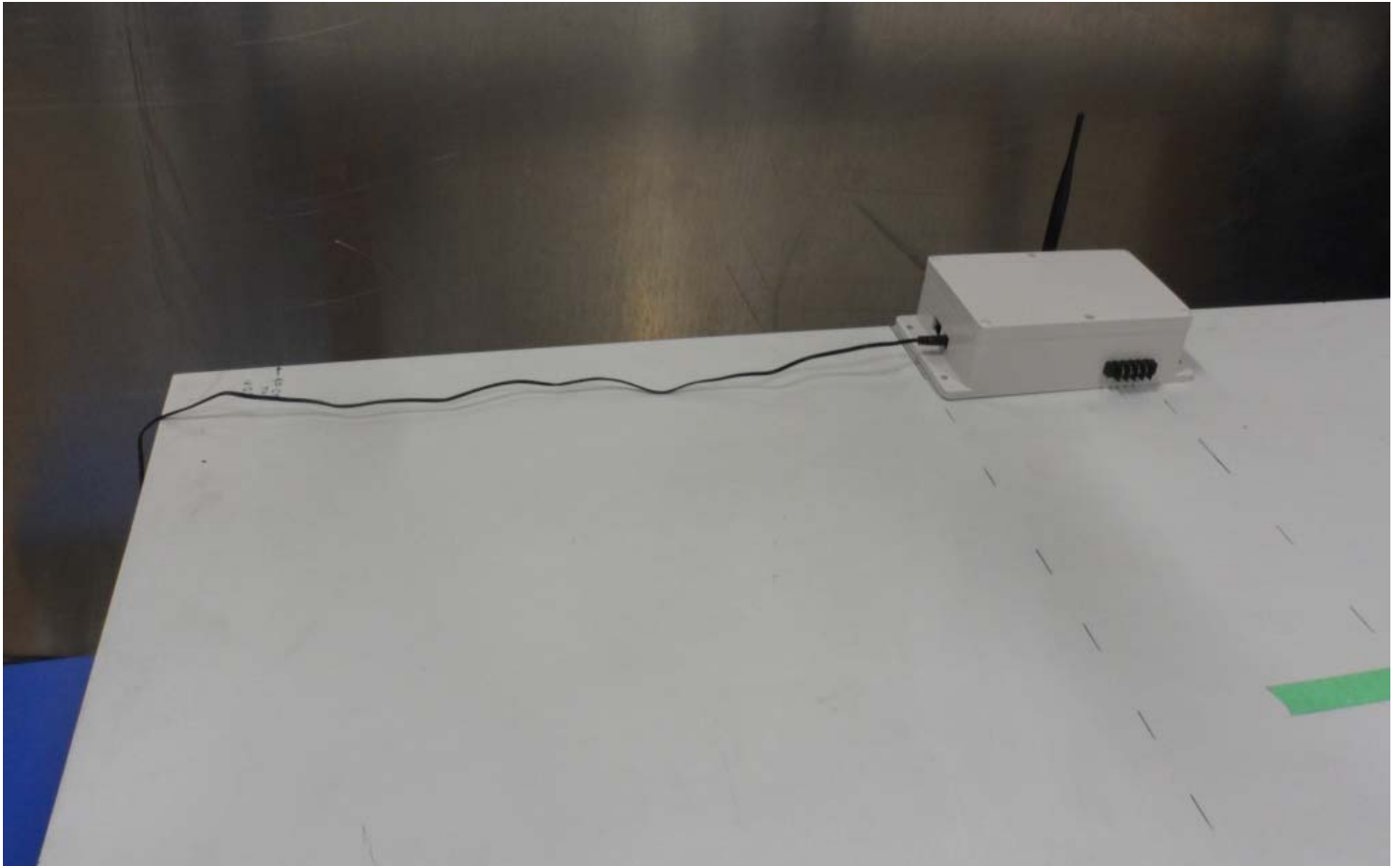
Figure E23.5 – Setup Photo – Power Line Conducted Measurements
