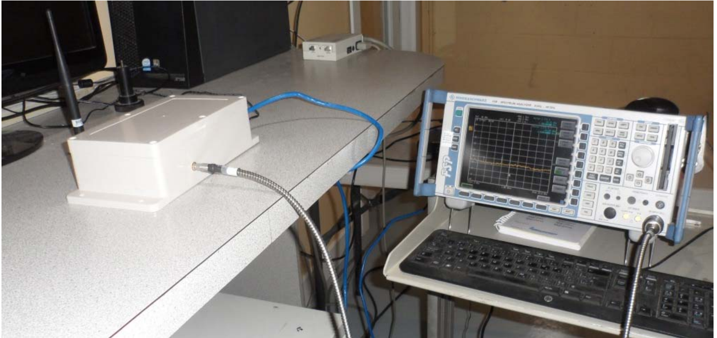
Figure E23.1 – Setup Photo – Conducted Measurements
