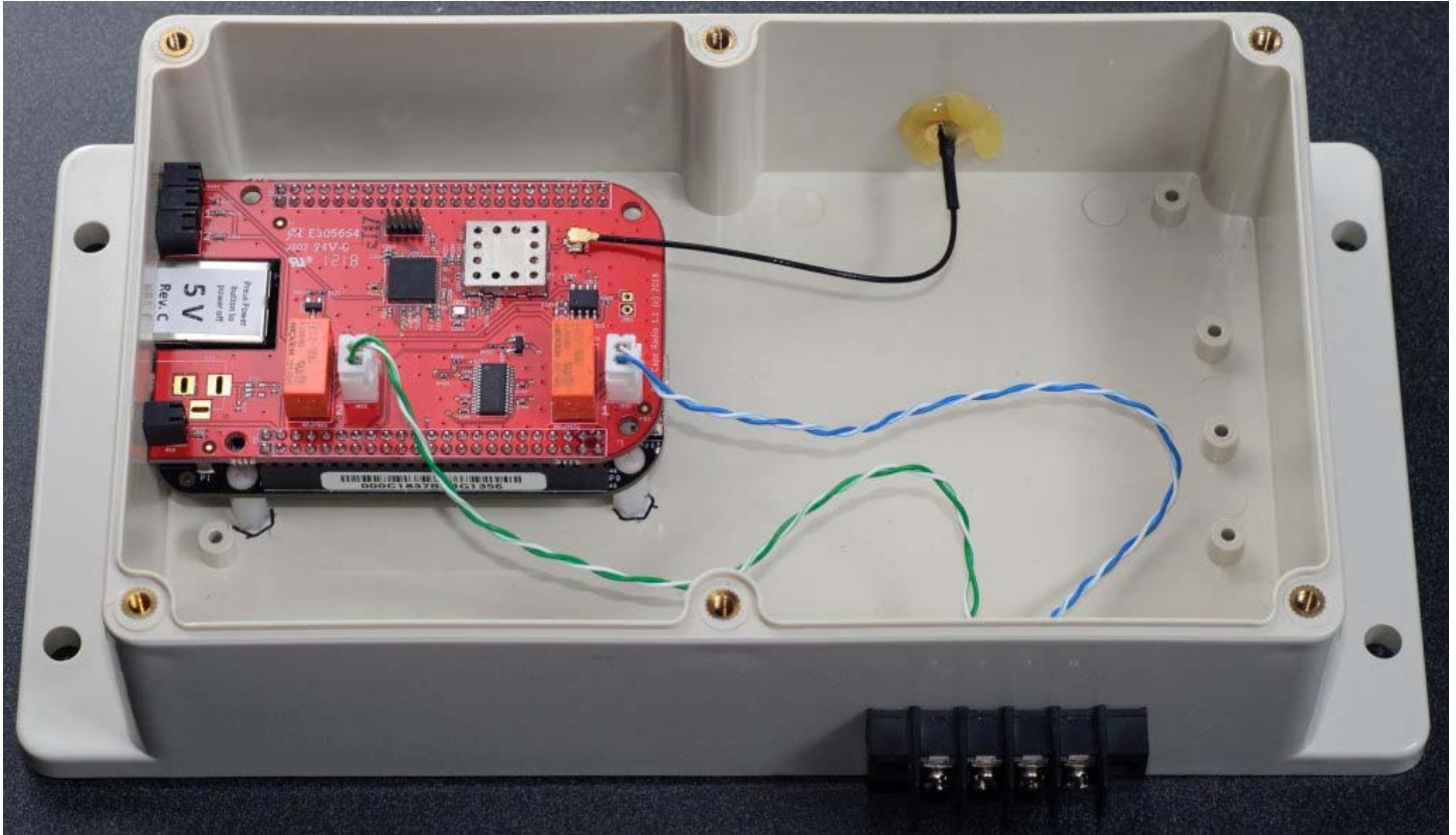
Figure E22.1 – Internal Photo – Host Internal
