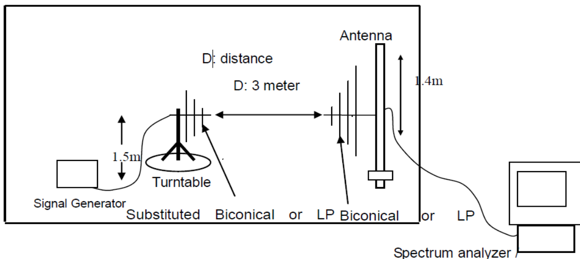
(A) Radiated Emission Test-Up Frequency Above 30MHz Ground Plane
