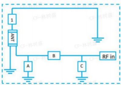
3216 Chip Antenna
