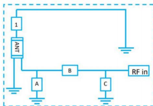
3216 Chip Antenna
