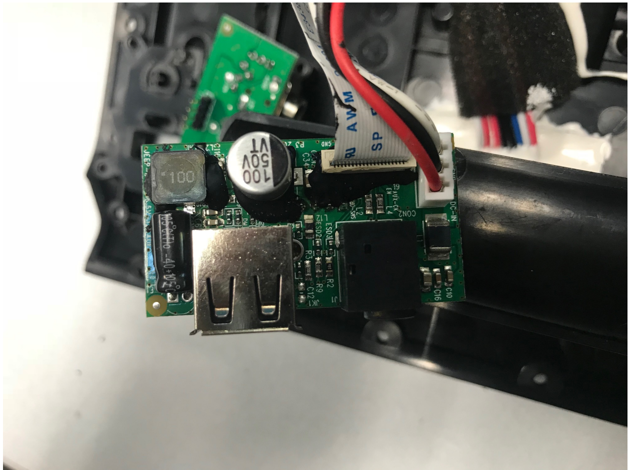
IO-PWR board top
