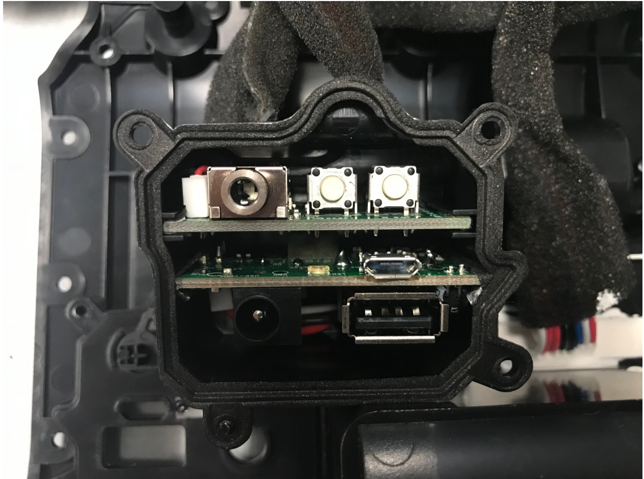
IO-AUD and IO-PWR board mounting
