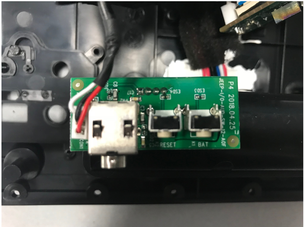
IO-AUD board top
