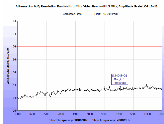
Plot 10. Radiated Emissions, 2402 MHz, 1 - 7 GHz, Peak, Horizontal
