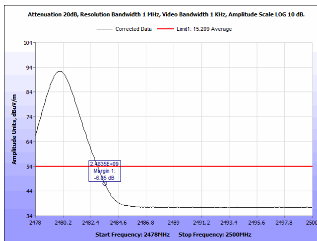
Plot 48. Radiated Restricted Bandedge, 2480 MHz, Average, Horizontal
