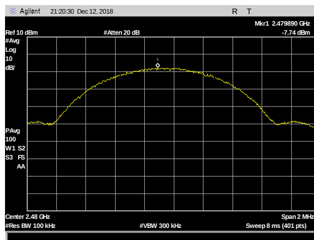
Plot 59. Power Density, 2480 MHz, 100 kHz RBW
