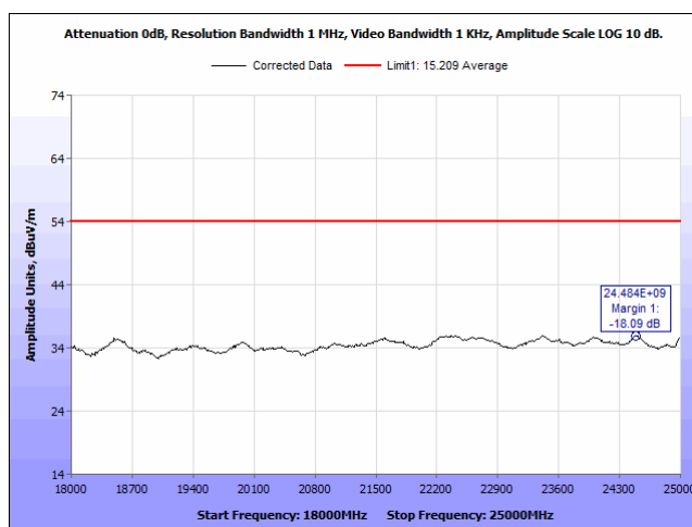
Plot 29. Radiated Emissions, 2440 MHz, 18 - 25 GHz, Average, Vertical
