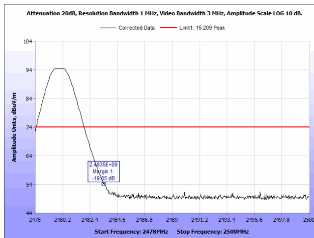
Plot 46. Radiated Restricted Bandedge, 2480 MHz, Peak, Horizontal
