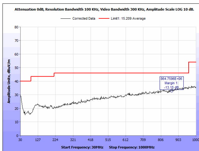
Plot 8. Radiated Emissions, 2402 MHz, 30 - 1000 MHz, Horizontal
