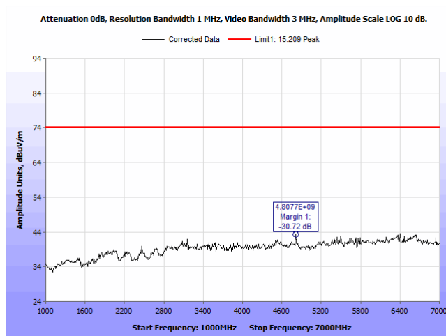
Plot 9. Radiated Emissions, 2402 MHz, 1 - 7 GHz, Peak, Vertical
