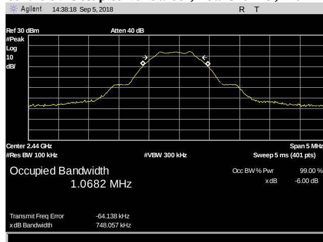
Plot 2. 6 dB Occupied Bandwidth, Mid Channel, 2440 MHz
