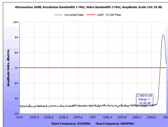
Plot 42. Radiated Restricted Bandedge, 2402 MHz, Peak, Horizontal
