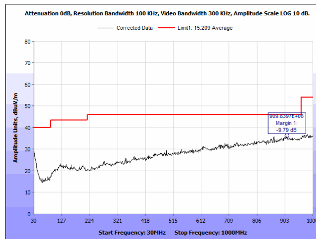
Plot 17. Radiated Emissions, 2440 MHz, 30 - 1000 MHz, Vertical
