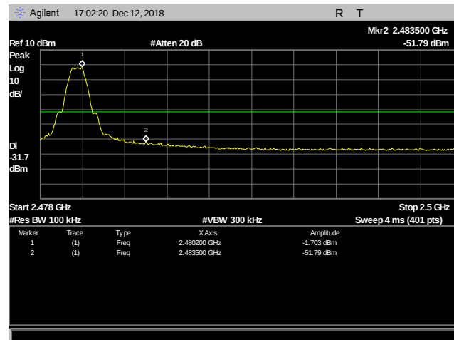
Plot 56. Conducted Restricted Bandedge, 2480 MHz
