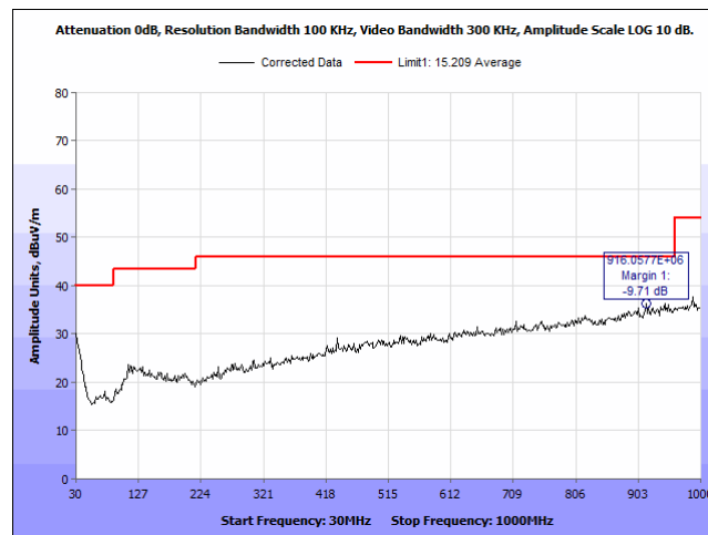
Plot 18. Radiated Emissions, 2440 MHz, 30 - 1000 MHz, Horizontal
