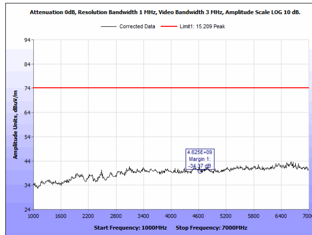
Plot 34. Radiated Emissions, 2480 MHz, 1 - 7 GHz, Peak, Horizontal
