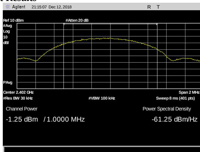
Plot 4. Maximum Conducted Output Power, 2402 MHz, Channel Power
