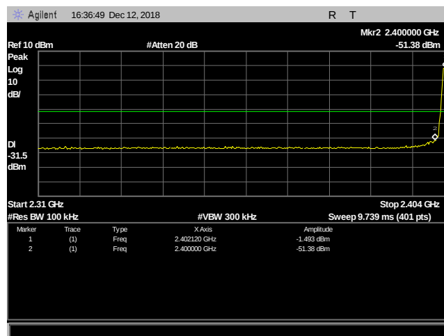
Plot 55. Conducted Restricted Bandedge, 2402 MHz
