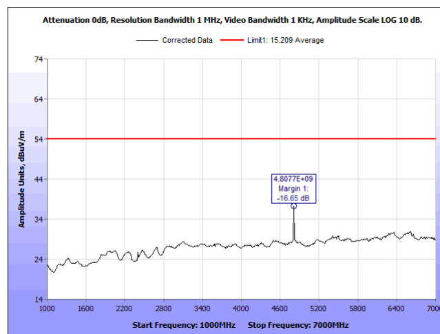
Plot 11. Radiated Emissions, 2402 MHz, 1 - 7 GHz, Average, Vertical
