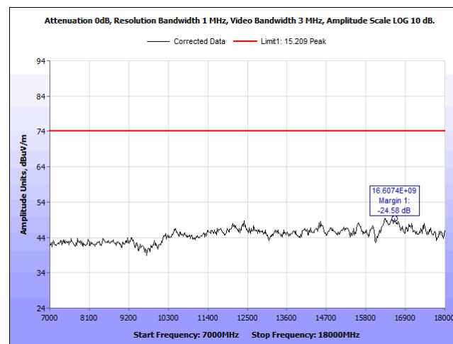
Plot 24. Radiated Emissions, 2440 MHz, 7 - 18 GHz, Peak, Horizontal
