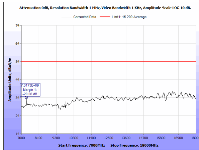
Plot 25. Radiated Emissions, 2440 MHz, 7 - 18 GHz, Average, Vertical
