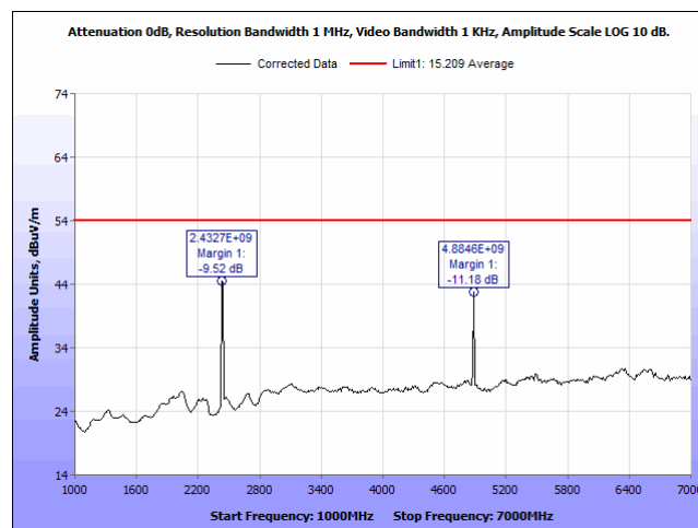
Plot 21. Radiated Emissions, 2440 MHz, 1 - 7 GHz, Average, Vertical
