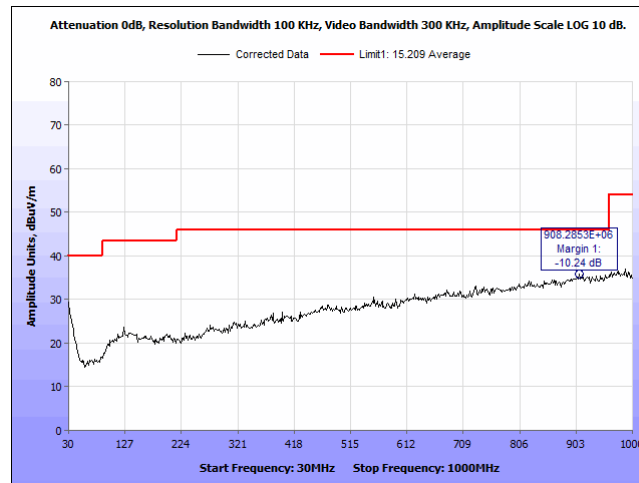
Plot 31. Radiated Emissions, 2480 MHz, 30 – 1000 MHz, Vertical
