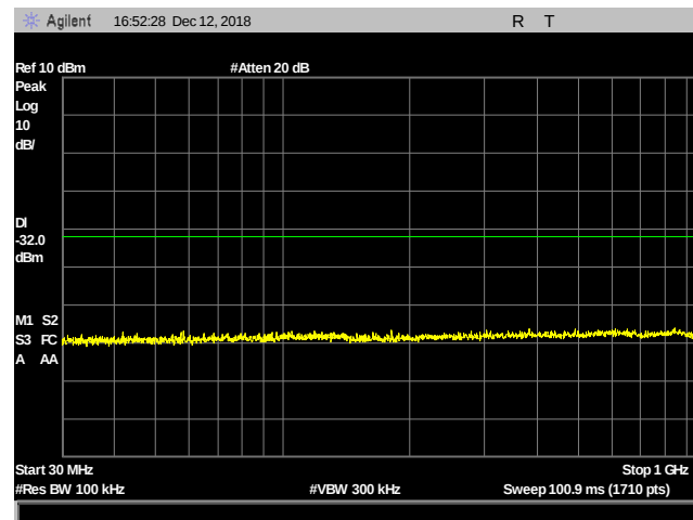
Plot 53. 100 kHz Spurious Emissions, 2480 MHz, 30 – 1000 MHz
