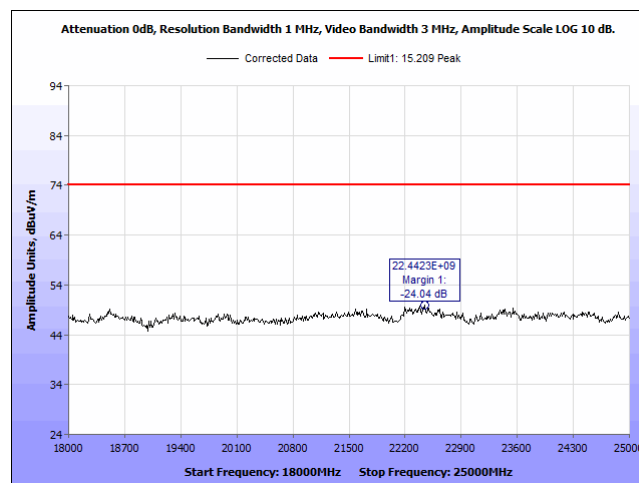
Plot 27. Radiated Emissions, 2440 MHz, 18 - 25 GHz, Peak, Vertical
