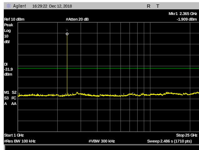
Plot 50. 100 kHz Spurious Emissions, 2402 MHz, 1 – 25 GHz
