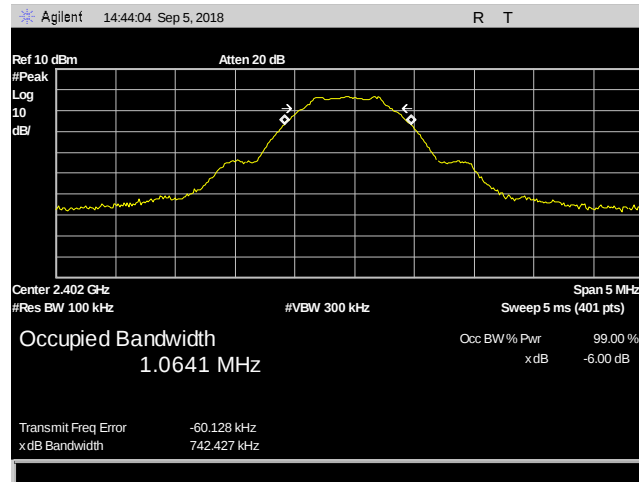
Plot 1. 6 dB Occupied Bandwidth, Low Channel, 2402 MHz
