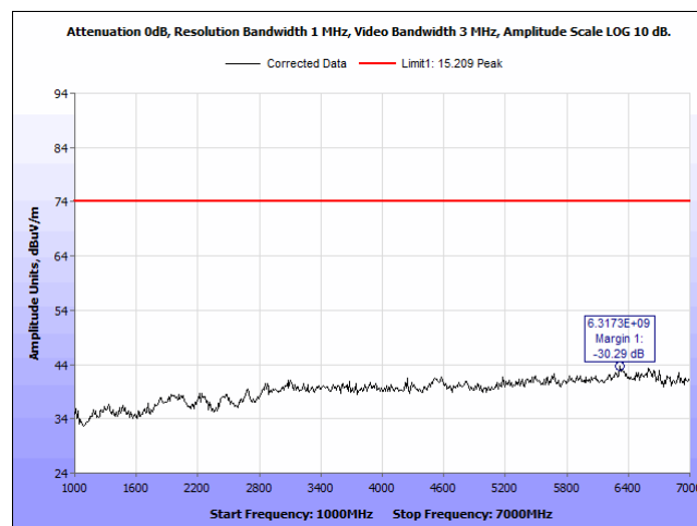
Plot 33. Radiated Emissions, 2480 MHz, 1 - 7 GHz, Peak, Vertical
