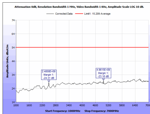
Plot 35. Radiated Emissions, 2480 MHz, 1 - 7 GHz, Average, Vertical
