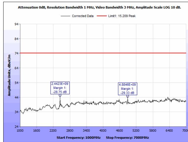
Plot 19. Radiated Emissions, 2440 MHz, 1 - 7 GHz, Peak, Vertical
