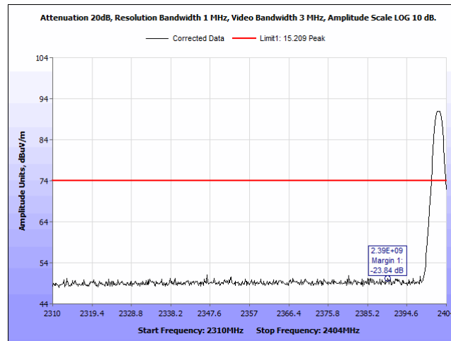
Plot 41. Radiated Restricted Bandedge, 2402 MHz, Peak, Vertical
