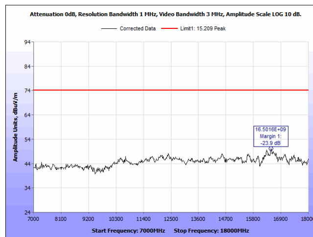
Plot 23. Radiated Emissions, 2440 MHz, 7 - 18 GHz, Peak, Vertical
