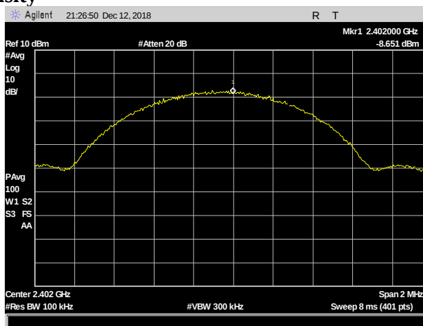
Plot 57. Power Density, 2402 MHz, 100 kHz RBW
