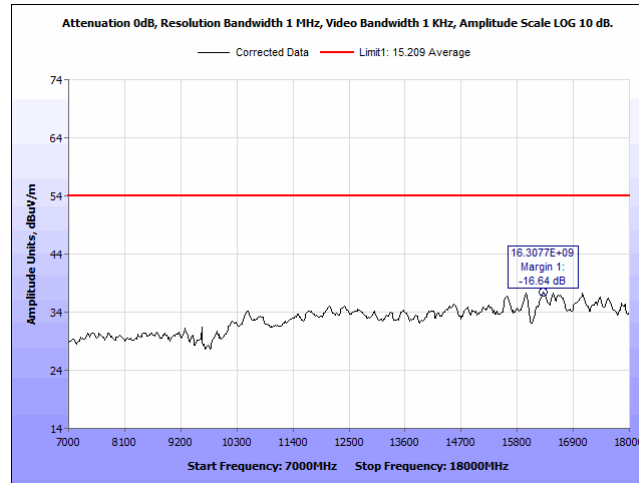
Plot 16. Radiated Emissions, 2402 MHz, 7 - 18 GHz, Average, Horizontal
