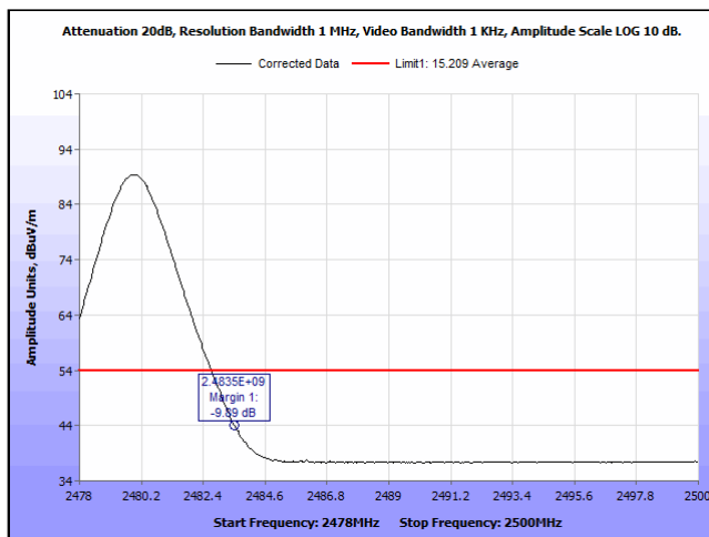
Plot 47. Radiated Restricted Bandedge, 2480 MHz, Average, Vertical
