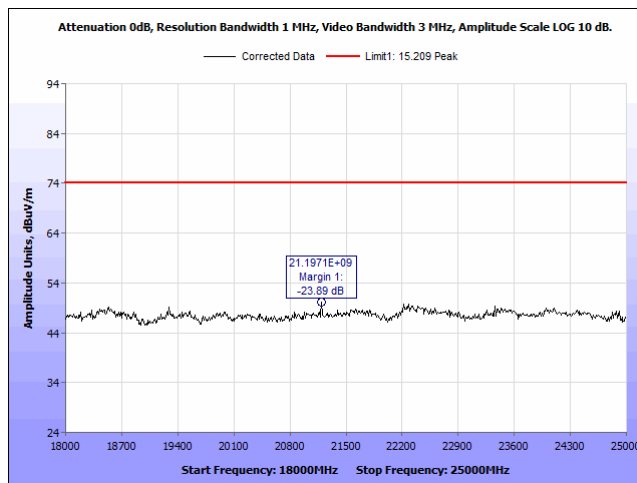
Plot 28. Radiated Emissions, 2440 MHz, 18 - 25 GHz, Peak, Horizontal
