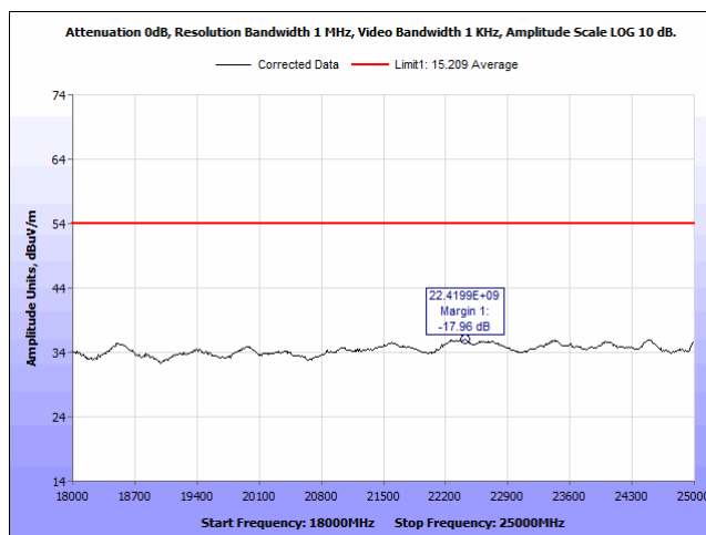
Plot 30. Radiated Emissions, 2440 MHz, 18 - 25 GHz, Average, Horizontal
