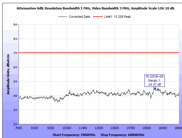
Plot 14. Radiated Emissions, 2402 MHz, 7 - 18 GHz, Peak, Horizontal
