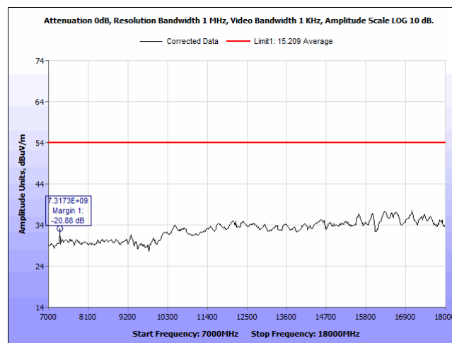
Plot 26. Radiated Emissions, 2440 MHz, 7 - 18 GHz, Average, Horizontal
