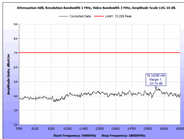
Plot 37. Radiated Emissions, 2480 MHz, 7 – 18 GHz, Peak, Vertical
