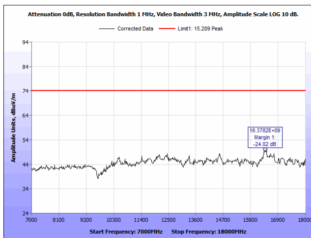
Plot 38. Radiated Emissions, 2480 MHz, 7 – 18 GHz, Peak, Horizontal
