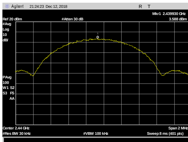
Plot 58. Power Density, 2440 MHz, 30 kHz RBW
