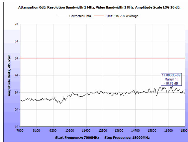
Plot 40. Radiated Emissions, 2480 MHz, 7 – 18 GHz, Average, Horizontal
