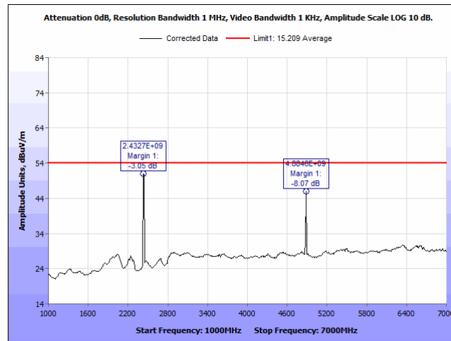
Plot 22. Radiated Emissions, 2440 MHz, 1 - 7 GHz, Average, Horizontal
