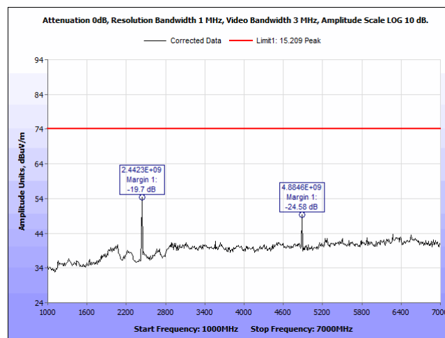
Plot 20. Radiated Emissions, 2440 MHz, 1 - 7 GHz, Peak, Horizontal
