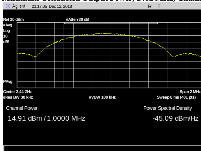
Plot 5. Maximum Conducted Output Power, 2440 MHz, Channel Power
