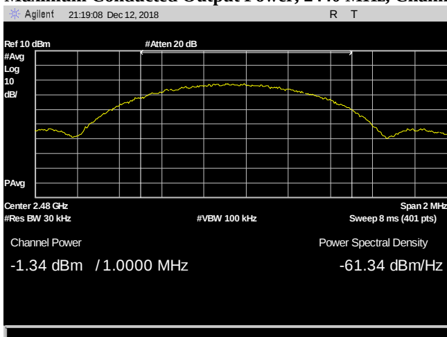
Plot 6. Maximum Conducted Output Power, 2480 MHz, Channel Power
