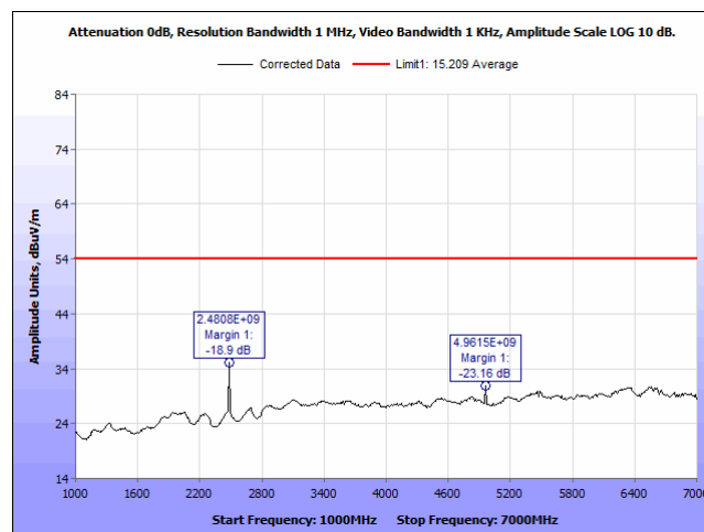
Plot 36. Radiated Emissions, 2480 MHz, 1 - 7 GHz, Average, Horizontal
