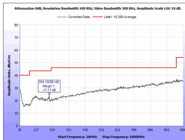
Plot 32. Radiated Emissions, 2480 MHz, 30 – 1000 MHz, Horizontal
