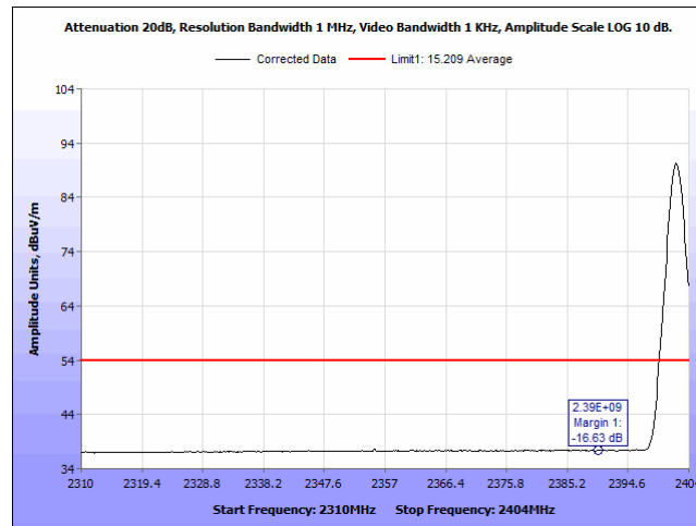
Plot 43. Radiated Restricted Bandedge, 2402 MHz, Average, Vertical
