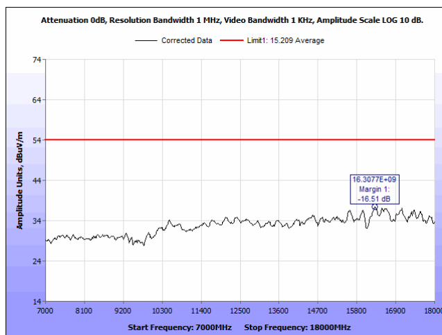
Plot 15. Radiated Emissions, 2402 MHz, 7 - 18 GHz, Average, Vertical
