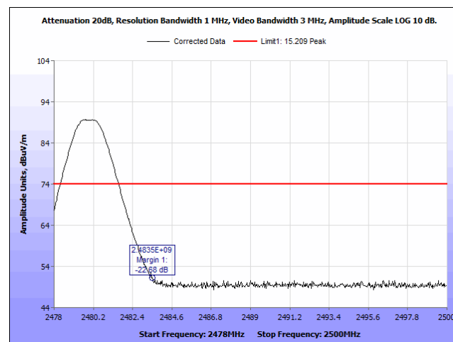
Plot 45. Radiated Restricted Bandedge, 2480 MHz, Peak, Vertical
