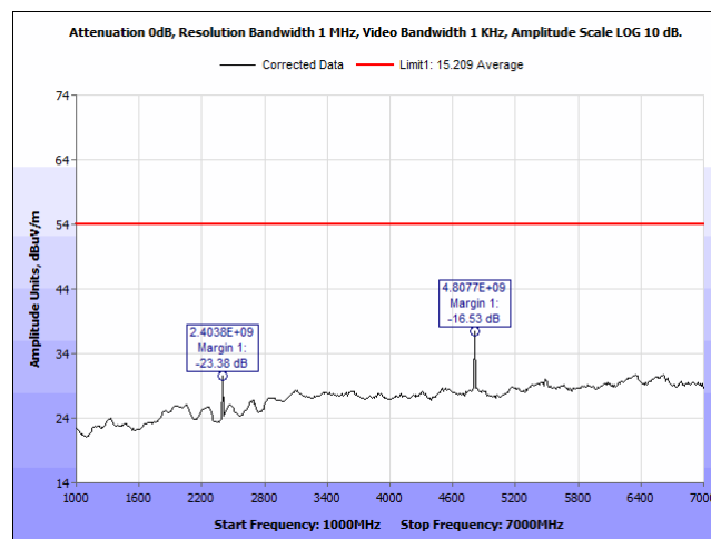
Plot 12. Radiated Emissions, 2402 MHz, 1 - 7 GHz, Average, Horizontal
