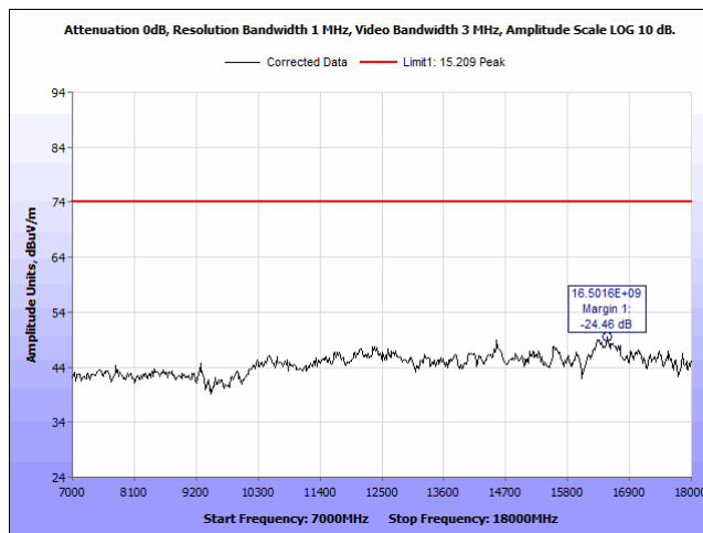
Plot 13. Radiated Emissions, 2402 MHz, 7 - 18 GHz, Peak, Vertical
