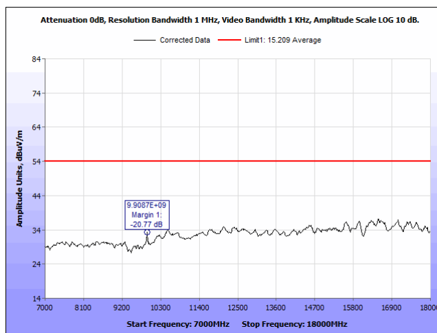
Plot 39. Radiated Emissions, 2480 MHz, 7 – 18 GHz, Average, Vertical
