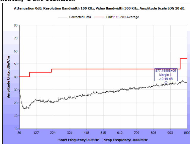
Plot 7. Radiated Emissions, 2402 MHz, 30 - 1000 MHz, Vertical
