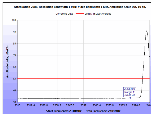
Plot 44. Radiated Restricted Bandedge, 2402 MHz, Average, Horizontal
