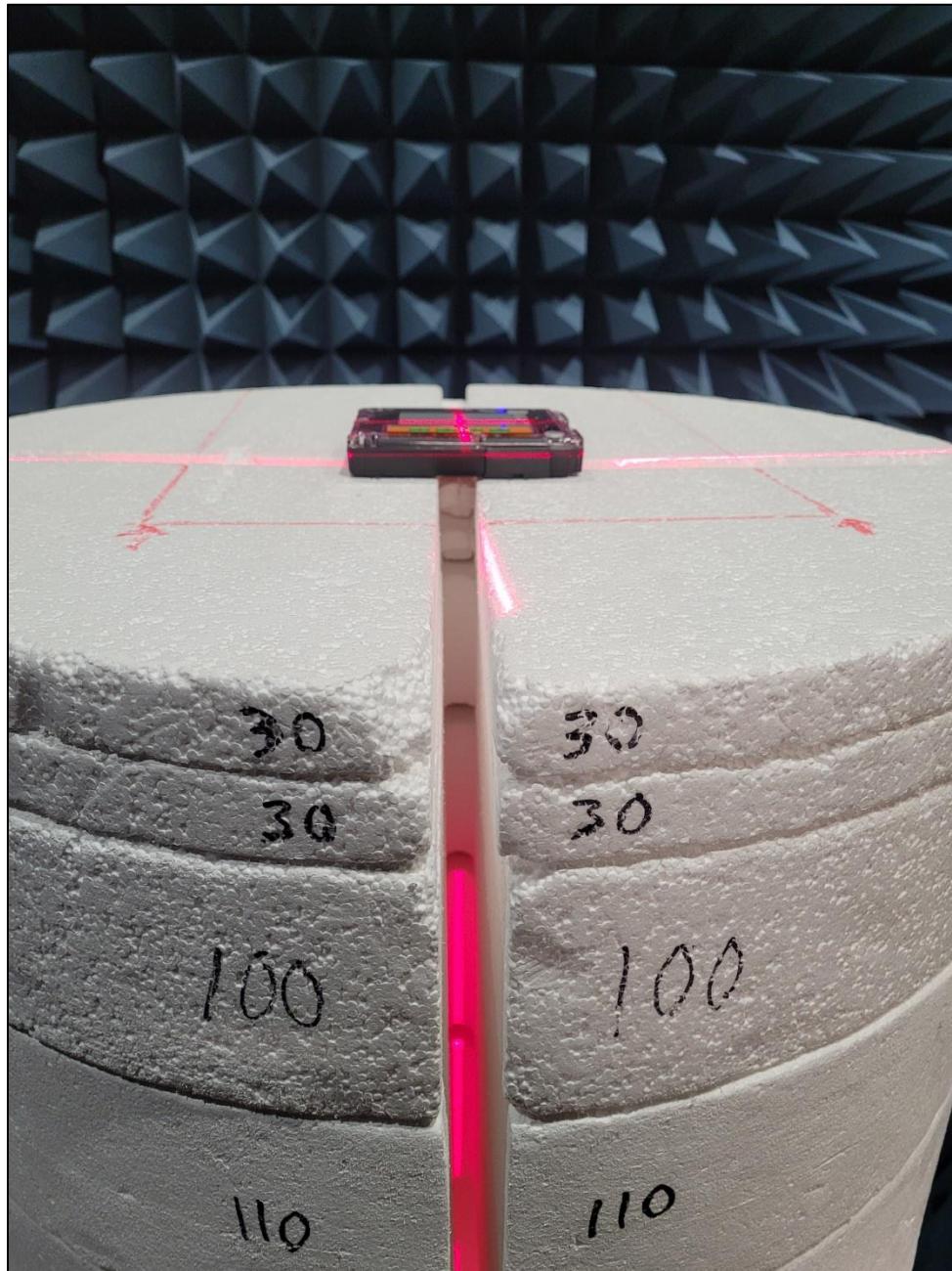
EIRP Measurement Test Setup View 2
