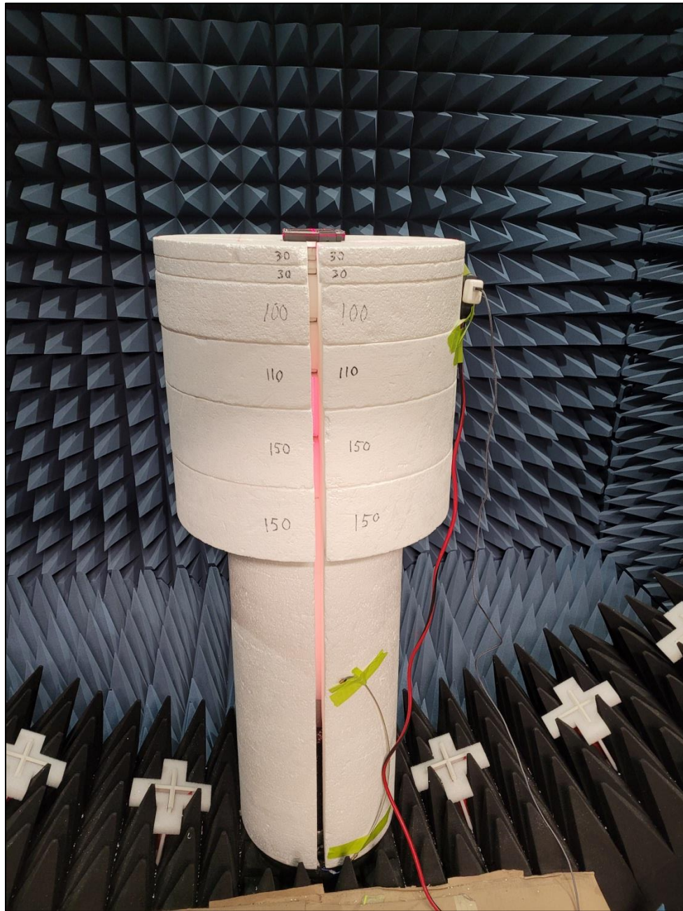
EIRP Measurement Test Setup View 1
