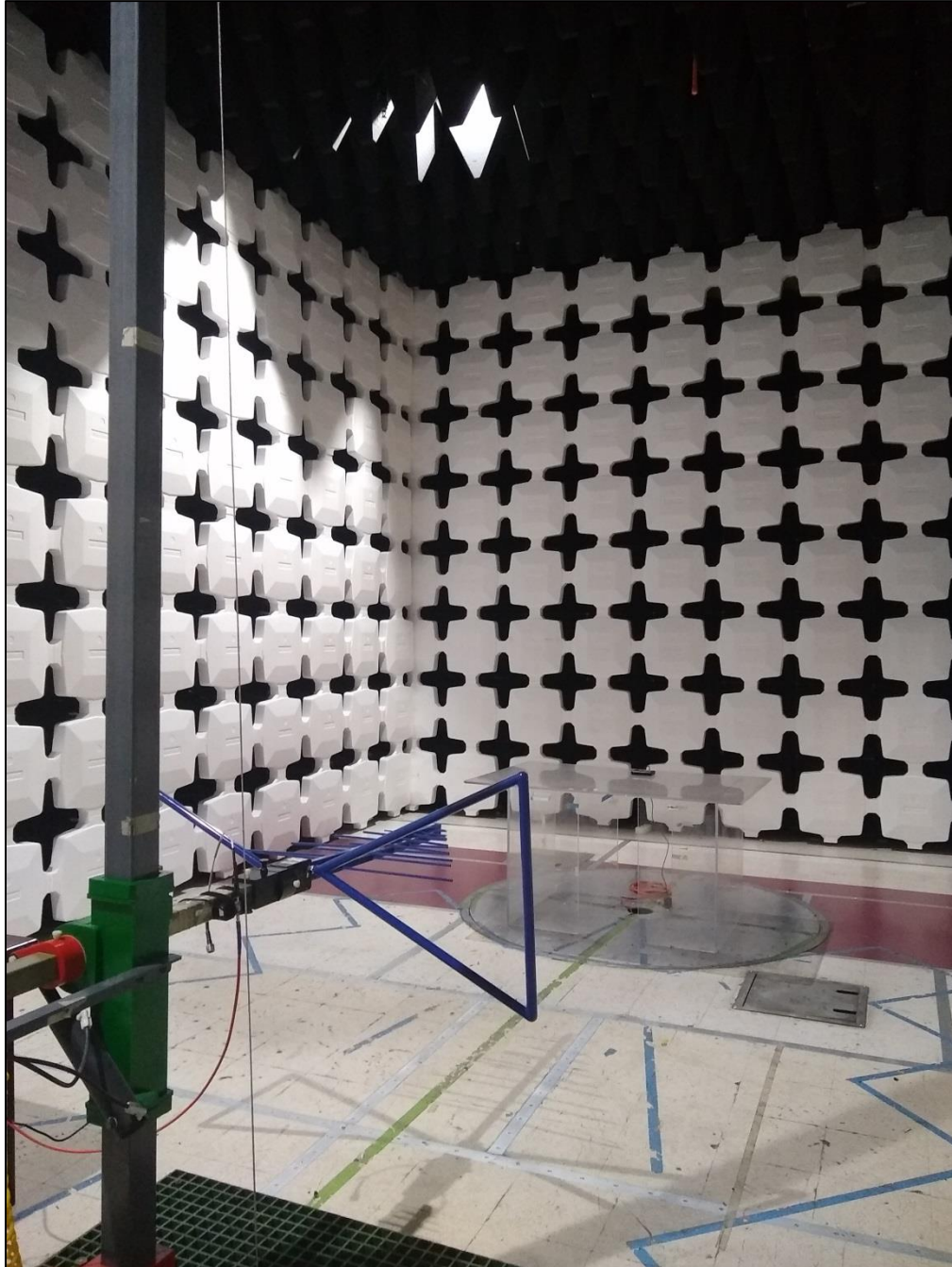
FCC Part 15B, 30MHz – 1GHz, Test Setup
