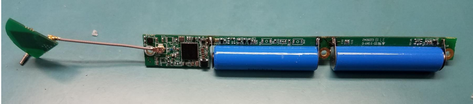
PCB Image Side A
