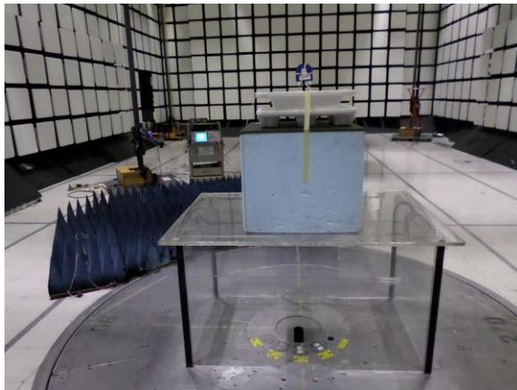
Figure 10: Radiated Emissions - 18GHz-25GHz - Setup Rear View
