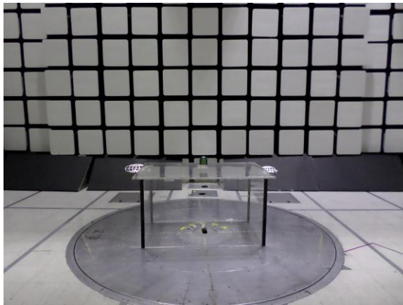
Figure 3: Radiated Emissions - 30MHz-1000MHz - Setup Front View
