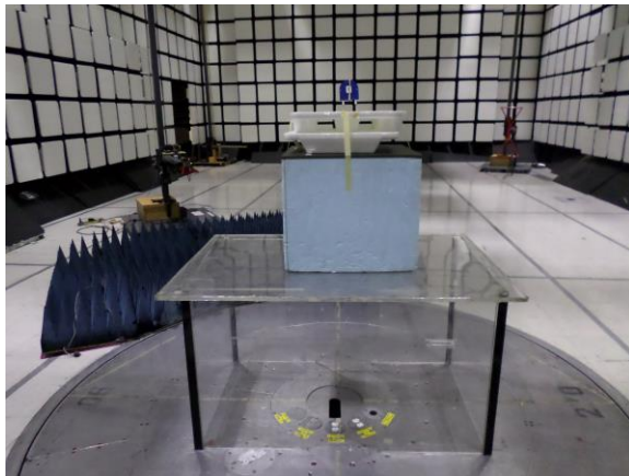
Figure 7: Radiated Emissions - 1GHz-18GHz - Setup Rear View
