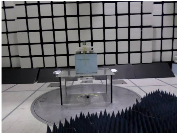
Figure 9: Radiated Emissions - 18GHz-25GHz - Setup Front View
