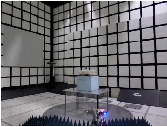
Figure 8: Radiated Emissions - 18GHz-25GHz - Setup Antenna View
