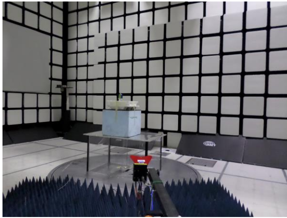
Figure 5: Radiated Emissions - 1GHz-18GHz - Setup Antenna View
