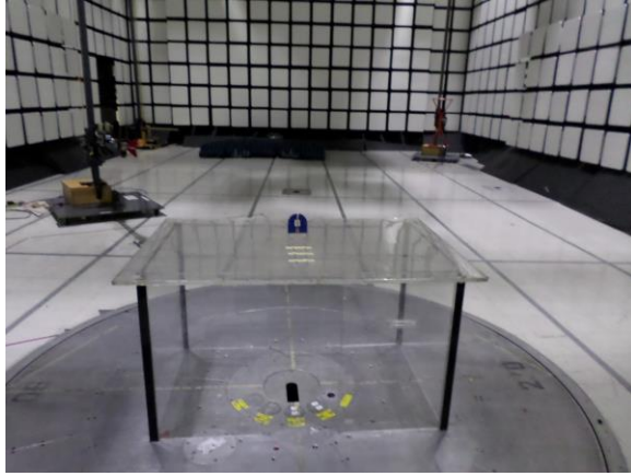
Figure 4: Radiated Emissions - 30MHz-1000MHz - Setup Rear View
