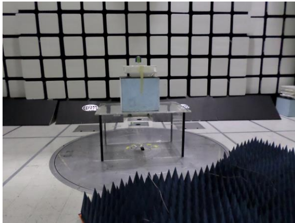
Figure 6: Radiated Emissions - 1GHz-18GHz - Setup Front View
