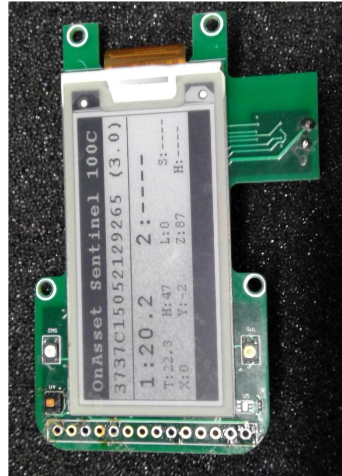
PCB2 Image Side B
