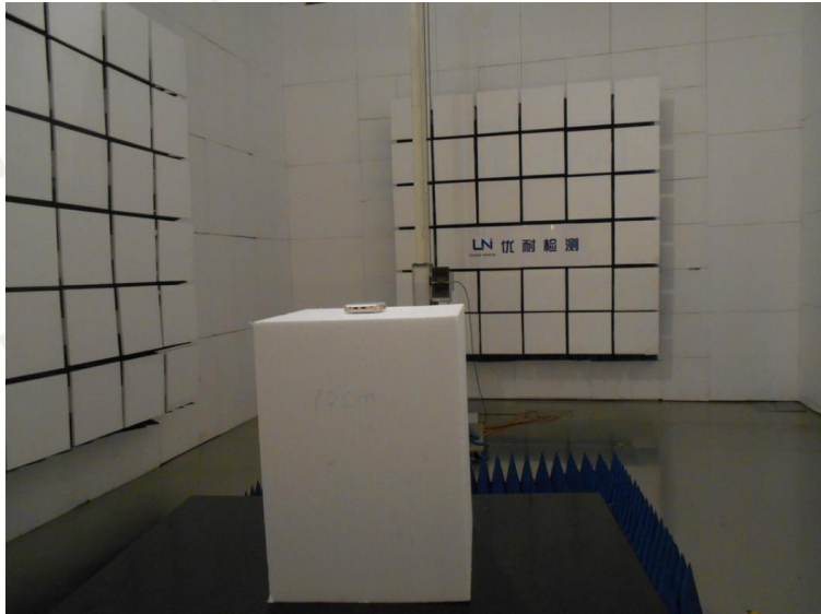
Radiated emission
