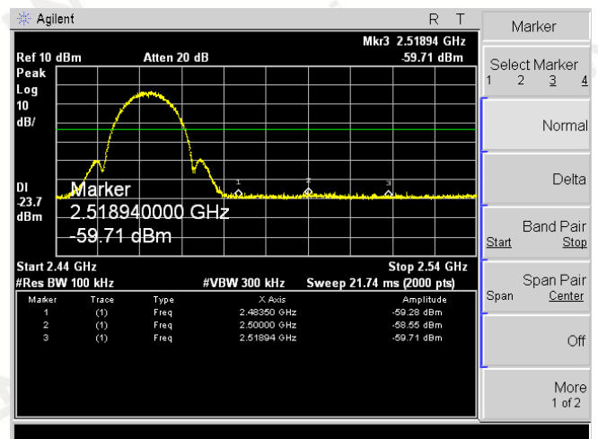
Right bandedge
