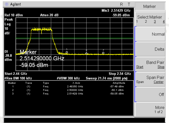
Right bandedge
