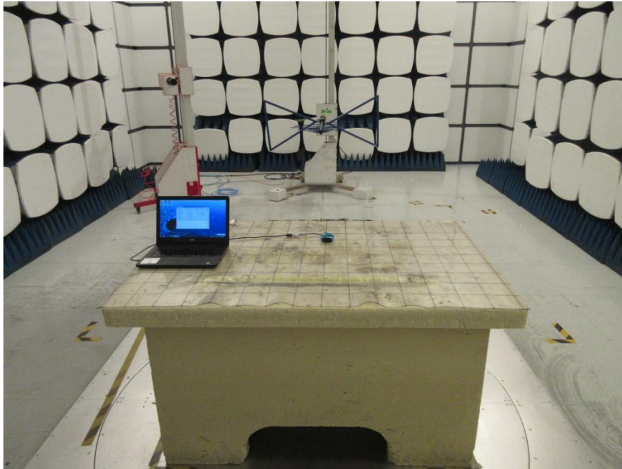
Radiation 30MHz-1GHz
