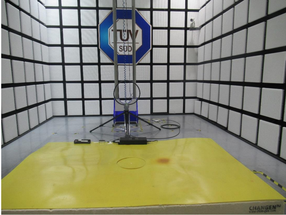
9KHz-30MHz Radiated Emission
