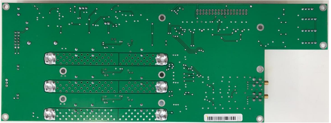
Bottom view
