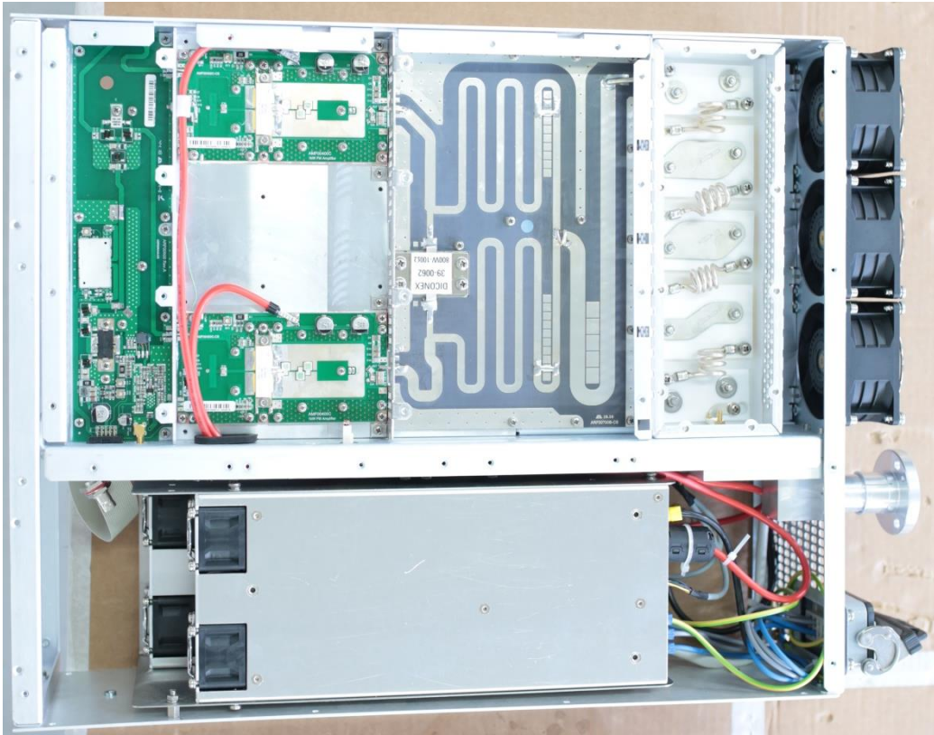
Bottom view
