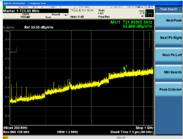
200-1000 MHz, Horizontal Polarity, BT 2402 MHz
