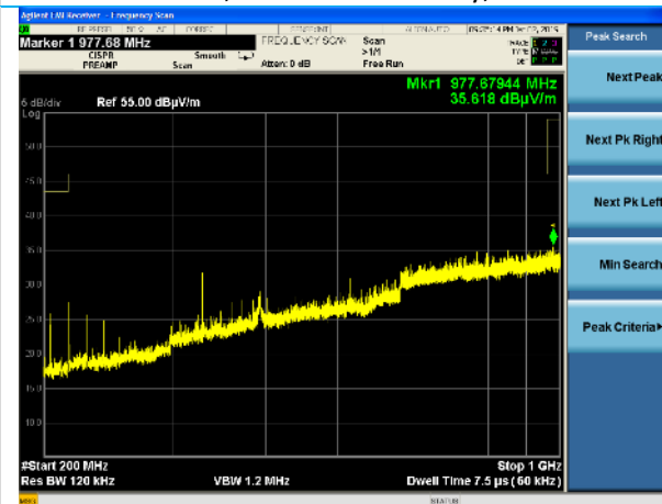
200-1000 MHz, Horizontal Polarity, BT 2480 MHz
