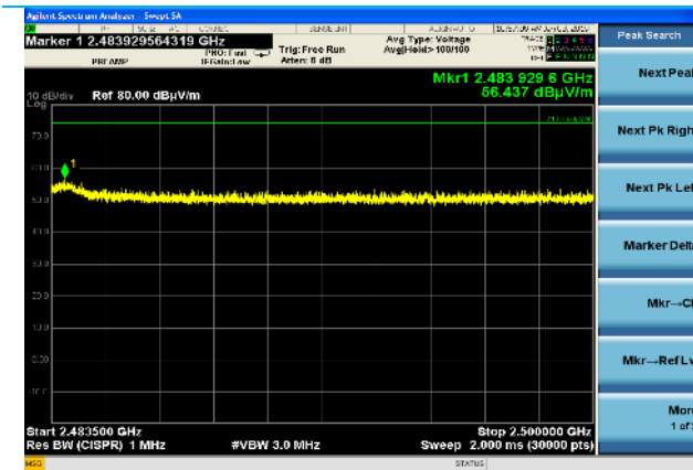
2483.5-2500 MHz, Peak Plot, BT 2480 MHz
