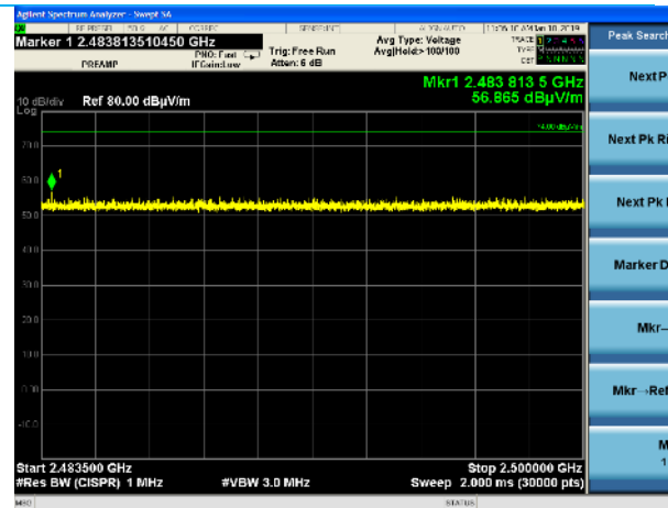
2483.5-2500 MHz, Peak Plot, BT Hopping GFSK
