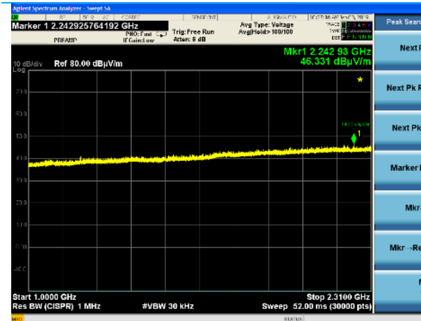
1000-2310 MHz, Vertical Polarity, BT 2402 MHz, Average Plot with Reduced VBW
