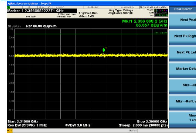
2310-2390 MHz, Peak Plot, BT 2402 MHz
