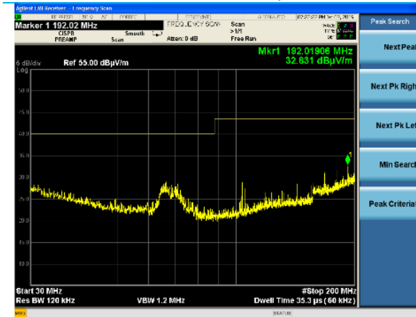
30-200 MHz, Vertical Polarity, BT 2480 MHz
