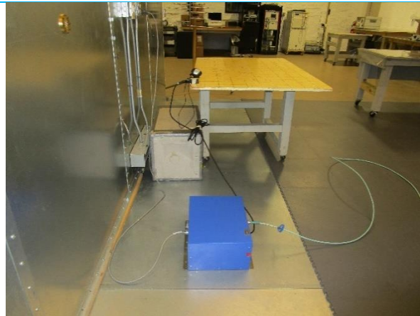
Conducted Emissions
