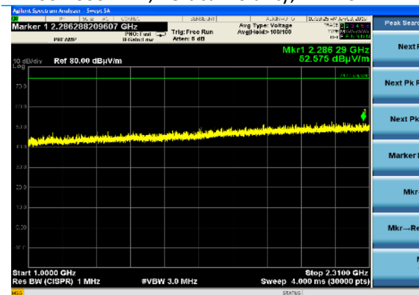
1000-2310 MHz, Vertical Polarity, BT 2402 MHz, Peak Plot
