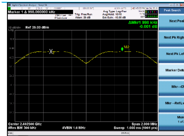
Separation, GFSK
