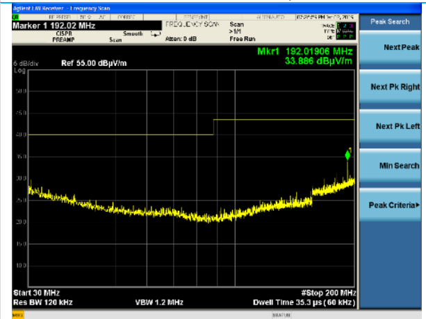
30-200 MHz, Horizontal Polarity, BT 2480 MHz
