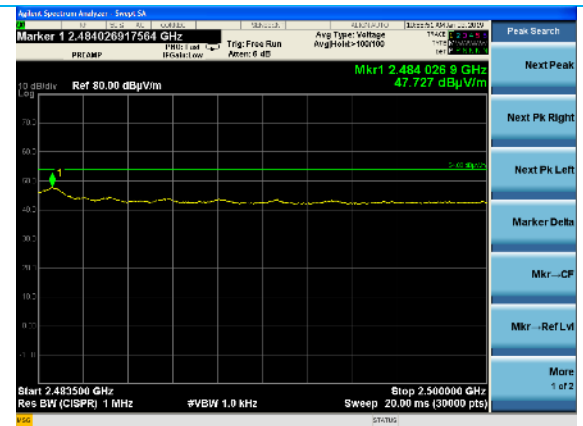
2483.5-2500 MHz, Average Plot, BT 2480 MHz, Reduced VBW
