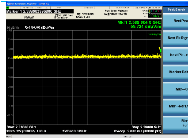
2310-2390 MHz, Peak Plot, BT Hopping GFSK
