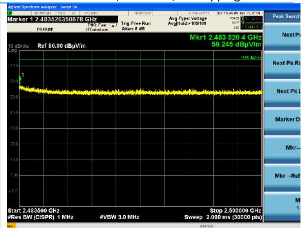
2483.5-2500 MHz, Peak Plot, BT Hopping EDR3
