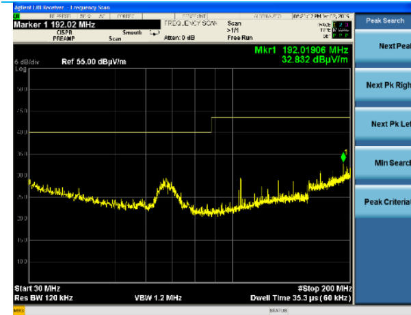
30-200 MHz, Vertical Polarity, BT 2402 MHz
