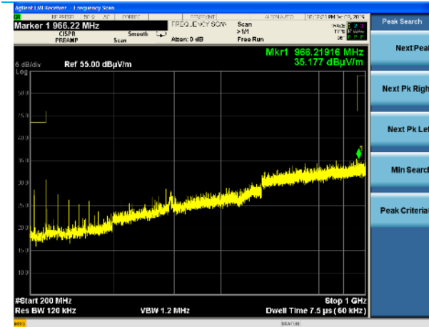
200-1000 MHz, Vertical Polarity, BT 2402 MHz
