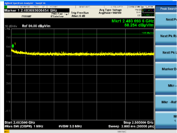
2483.5-2500 MHz, Peak Plot, BT Hopping EDR2
