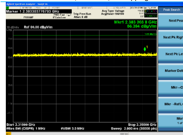
2310-2390 MHz, Peak Plot, BT Hopping EDR3
