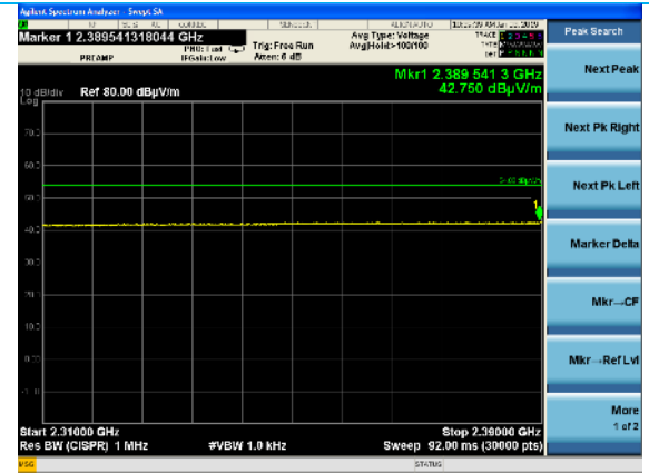
2310-2390 MHz, Average Plot, BT 2402 MHz, Reduced VBW
