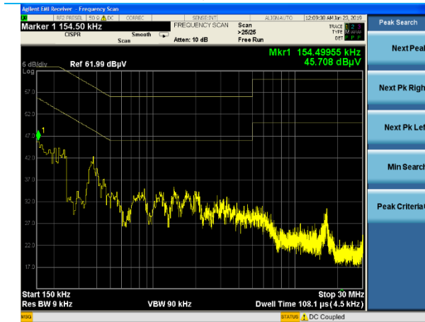
Line 1, 2480 MHz
