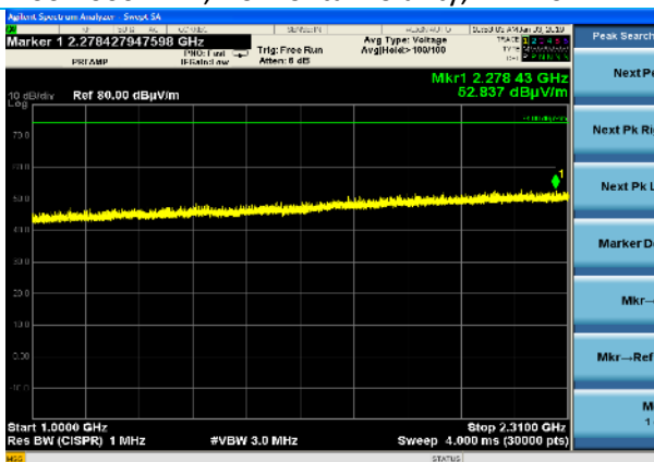
1000-2310 MHz, Vertical Polarity, BT 2480 MHz, Peak Plot
