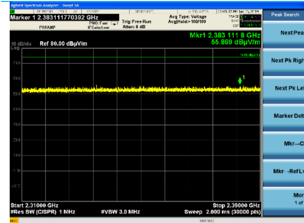
2310-2390 MHz, Peak Plot, BT Hopping EDR2
