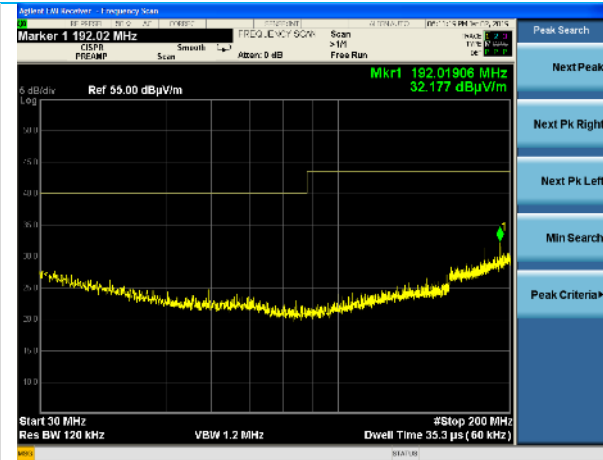
30-200 MHz, Horizontal Polarity, BT 2402 MHz
