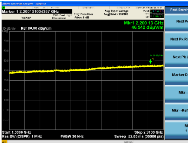
1000-2310 MHz, Vertical Polarity, BT 2480 MHz, Average Plot with Reduced VBW
