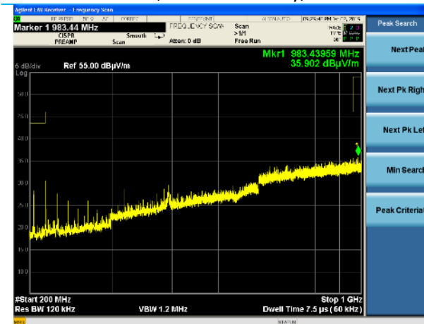
200-1000 MHz, Vertical Polarity, BT 2480 MHz
