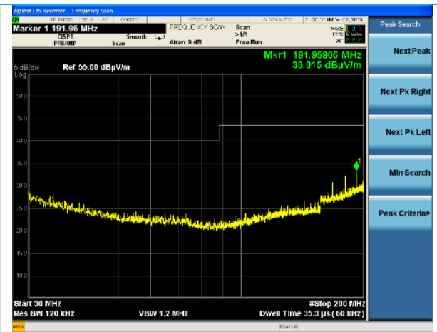
30-200 MHz, Horizontal Polarity, BT Disabled
