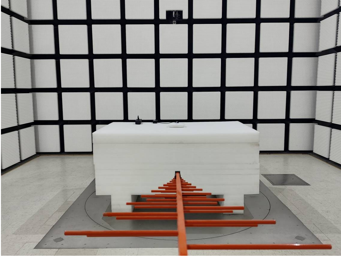
Radiated Emission Below 1GHz View- POE Power
