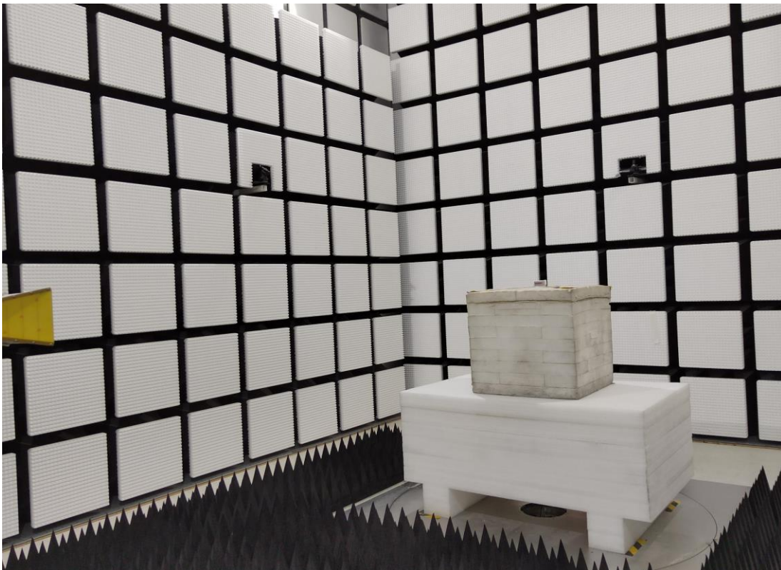
Radiated Emission Above 1GHz View
