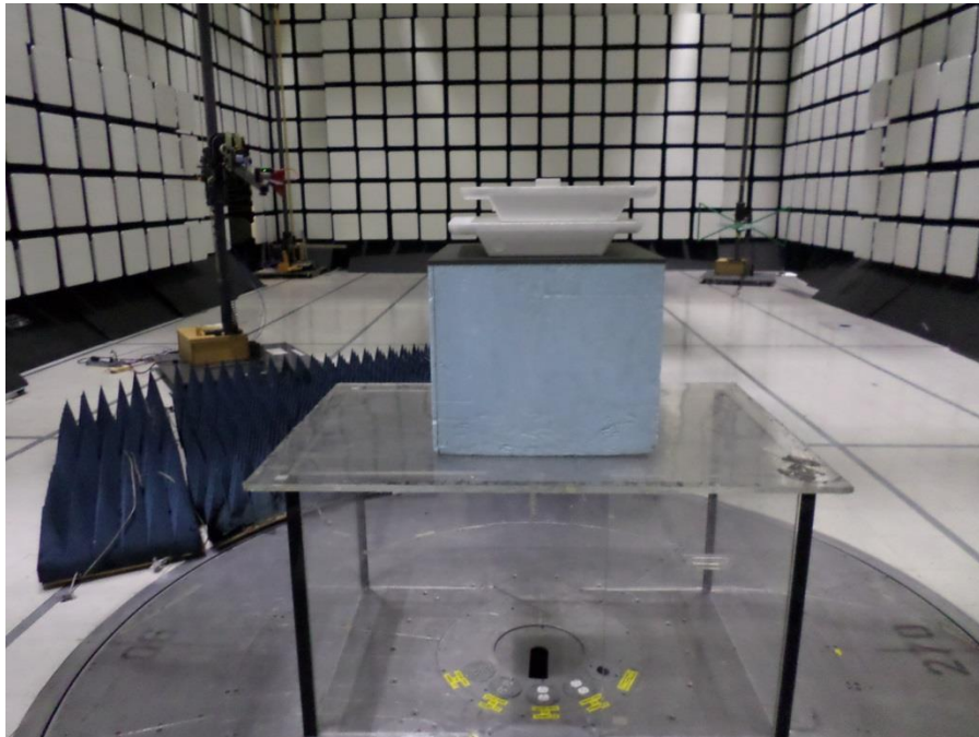
Photograph 6. Radiated Spurious Emissions, Above 1 GHz, Rear, Test Setup
