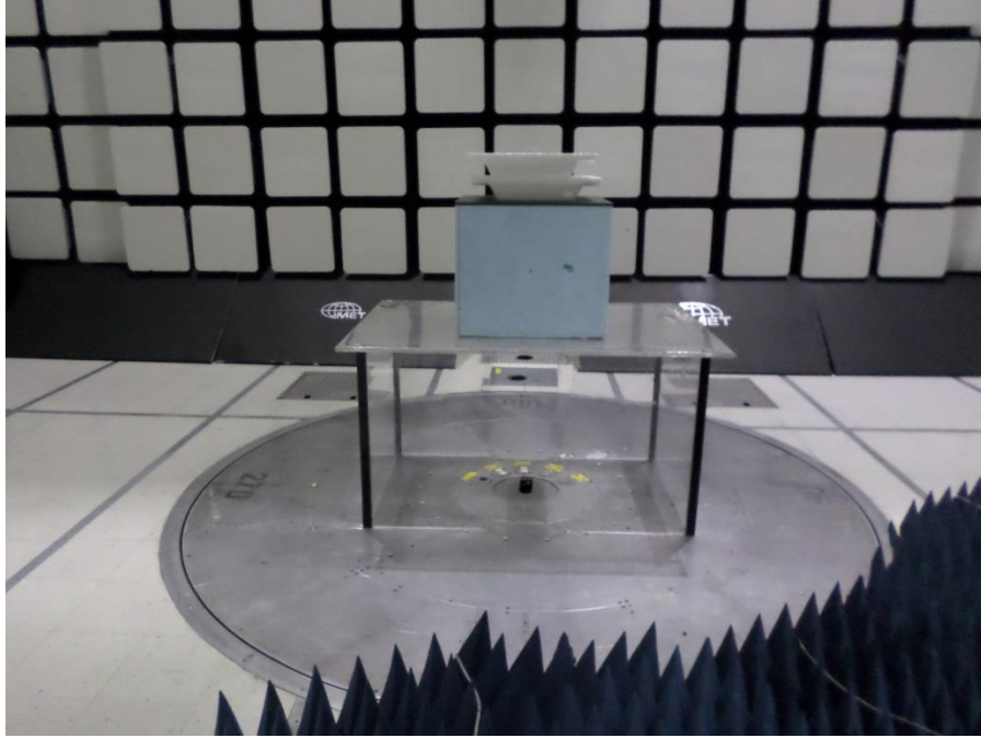
Photograph 5. Radiated Spurious Emissions, Above 1 GHz, Front, Test Setup
