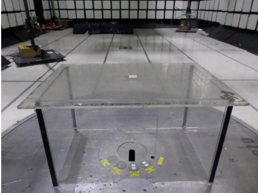
Photograph 3. Radiated Spurious Emissions, Below 1 GHz, Rear, Test Setup
