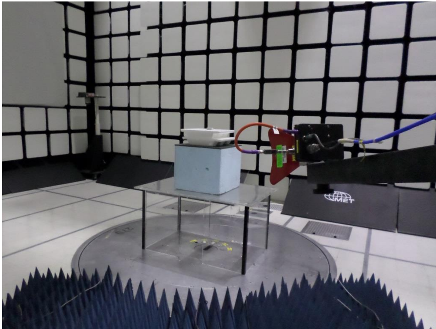
Photograph 4. Radiated Spurious Emissions, Above 1 GHz, Antenna, Test Setup
