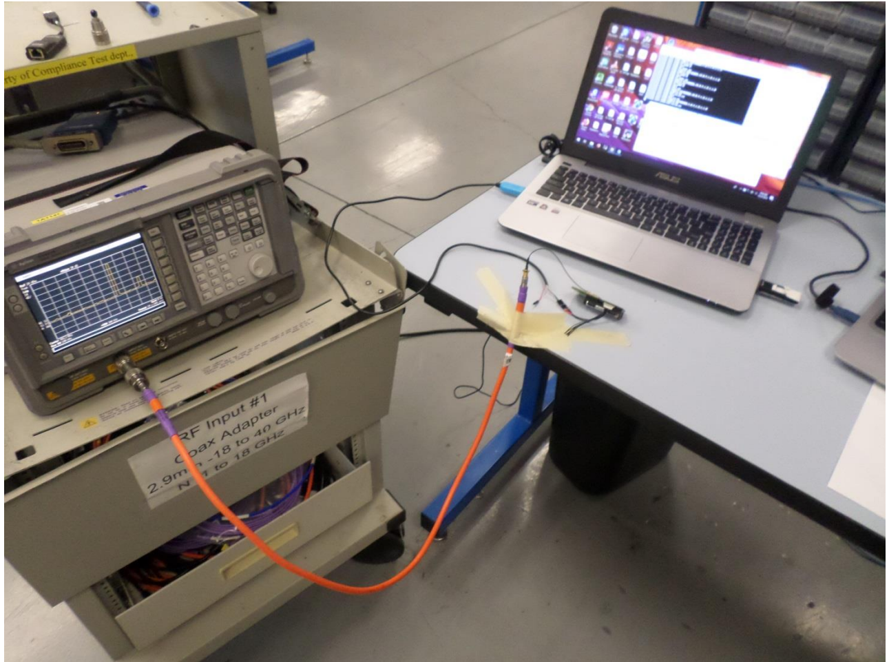
Photograph 7. Conducted Spurious Emissions, Test Setup
