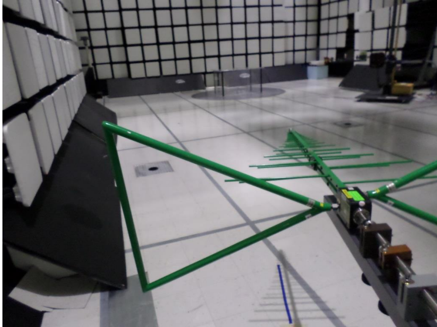
Photograph 1. Radiated Spurious Emissions, Below 1 GHz, Antenna, Test Setup
