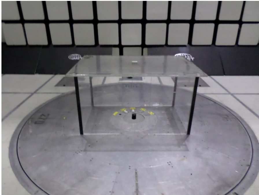
Photograph 2. Radiated Spurious Emissions, Below 1 GHz, Front, Test Setup
