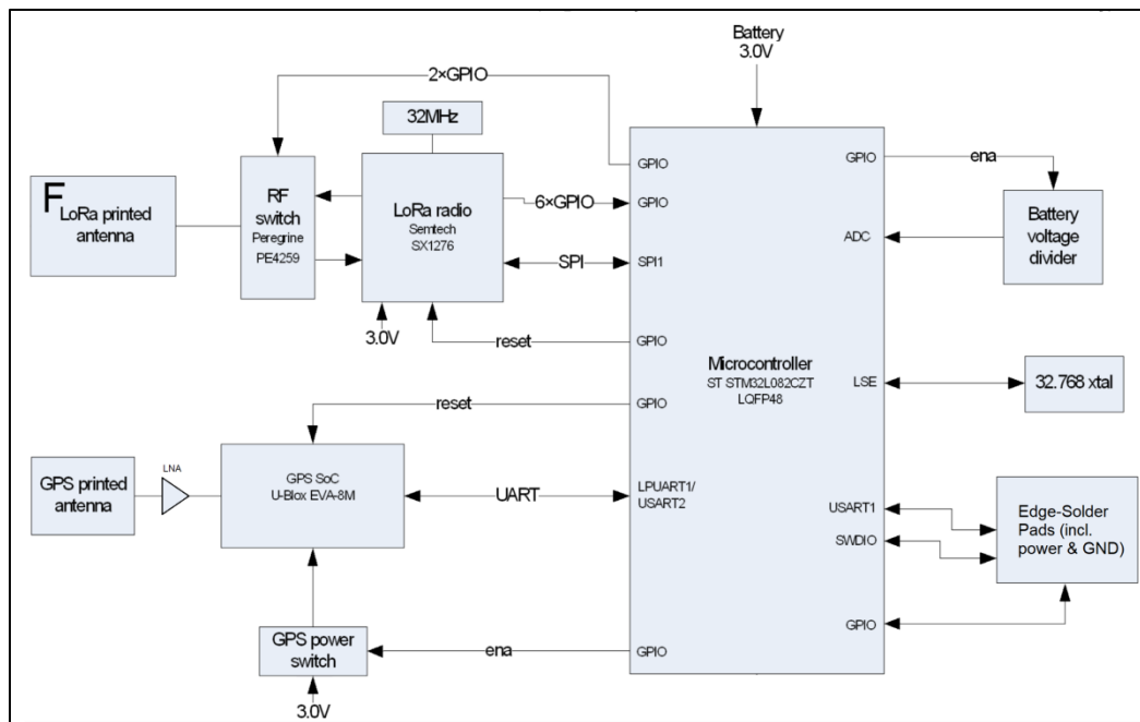
Figure 2. LoRa Module Block Diagram
