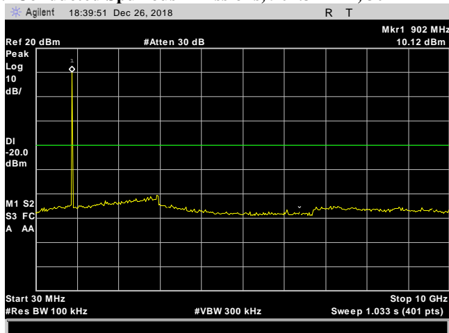
Plot 23. Conducted Spurious Emissions, 908.7 MHz, 30 MHz – 10 GHz
