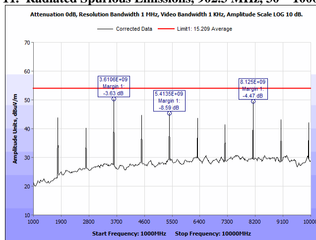
Plot 12. Radiated Spurious Emissions, 902.3 MHz, 1 – 10 GHz, Average
