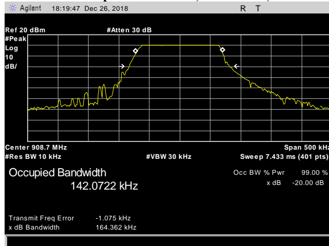
Plot 2. 20 dB Occupied Bandwidth, 908.7 MHz, 164.362 kHz
