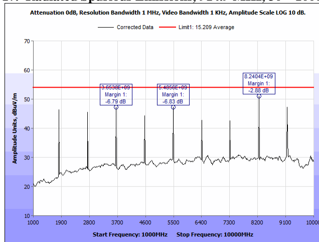
Plot 18. Radiated Spurious Emissions, 914.9 MHz, 1 – 10 GHz, Average
