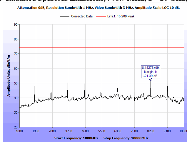
Plot 16. Radiated Spurious Emissions, 908.7 MHz, 1 – 10 GHz, Peak
