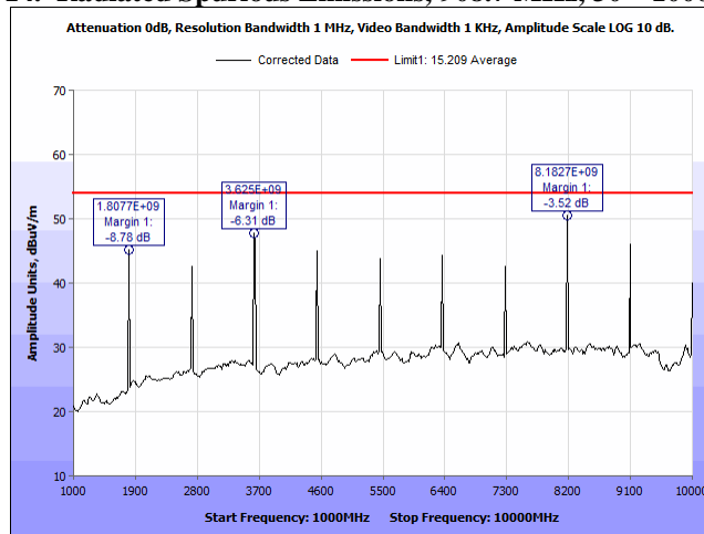
Plot 15. Radiated Spurious Emissions, 908.7 MHz, 1 – 10 GHz, Average
