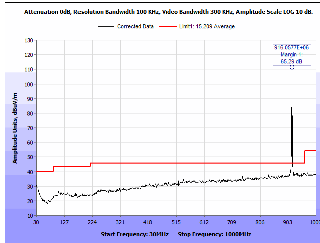
Plot 17. Radiated Spurious Emissions, 914.9 MHz, 30 – 1000 MHz
