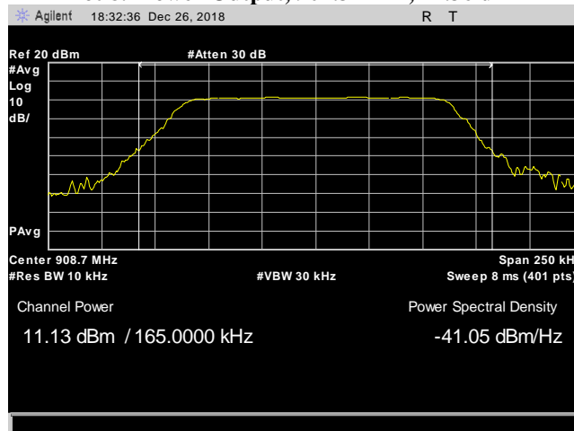
Plot 9. Power Output, 908.7 MHz, 11.13 dBm
