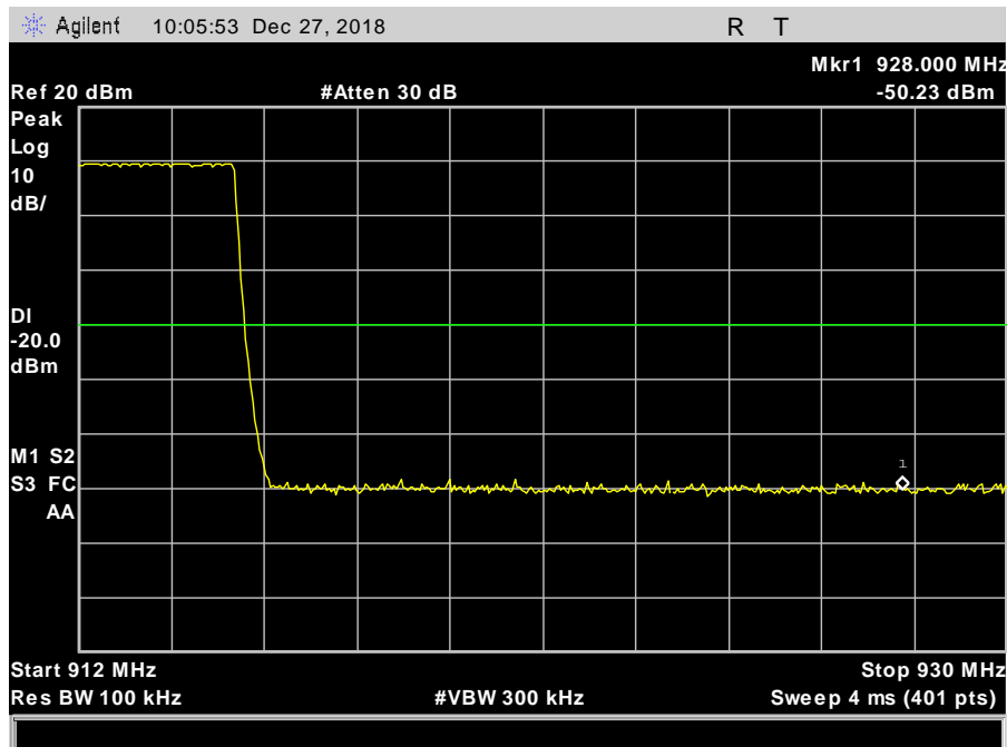
Plot 28. Conducted Band Edge, Hopping, High
