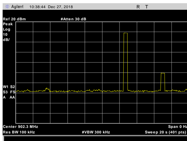
Plot 4. Dwell Time, 20s
