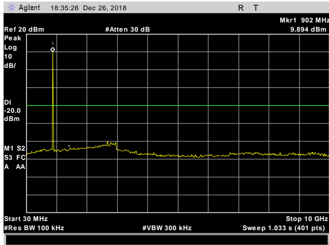
Plot 22. Conducted Spurious Emissions, 902.3 MHz, 30 MHz – 10 GHz
