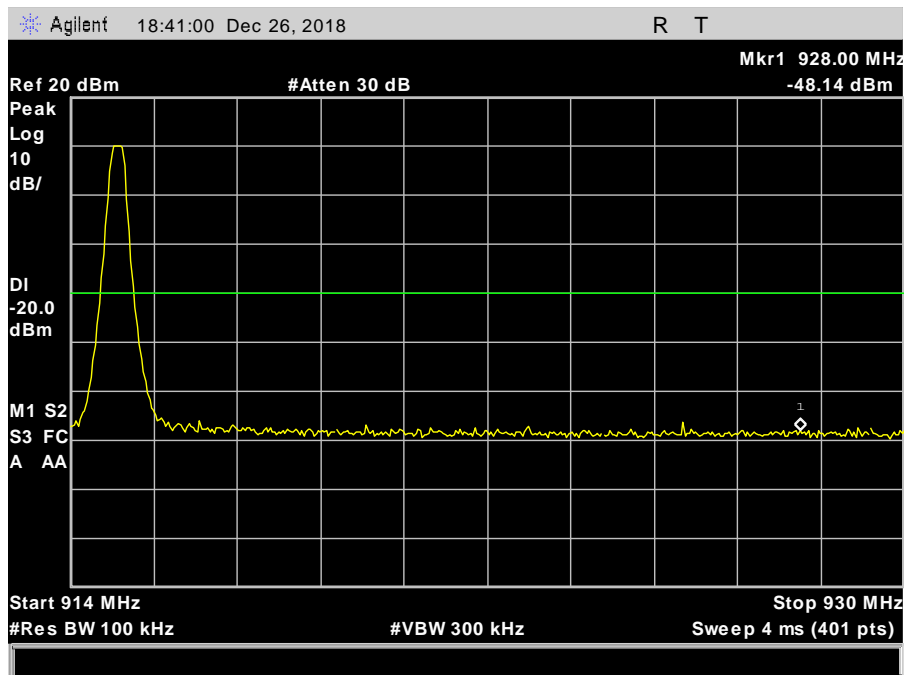
Plot 26. Conducted Band Edge, 914.9 MHz
