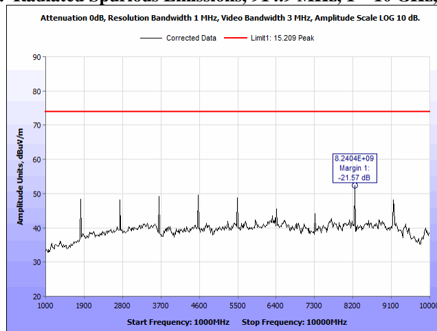
Plot 19. Radiated Spurious Emissions, 914.9 MHz, 1 – 10 GHz, Peak
