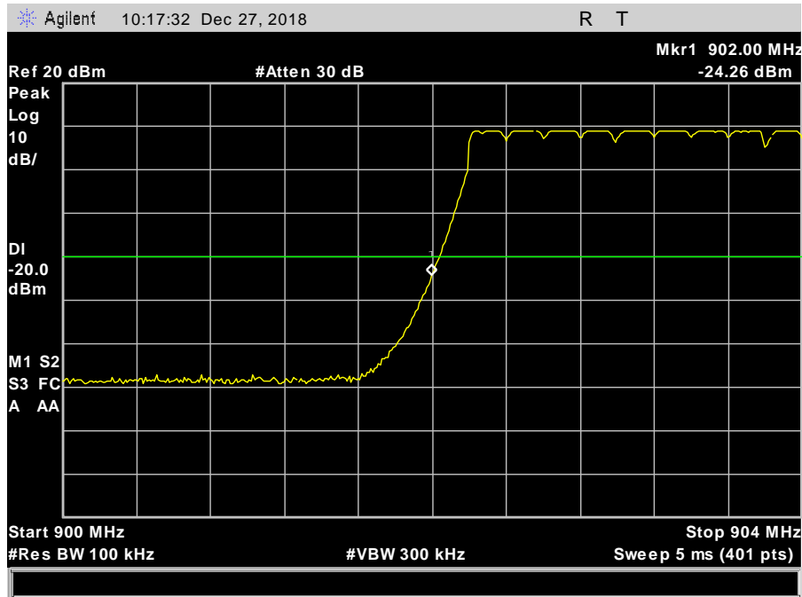
Plot 27. Conducted Band Edge, Hopping, Low
