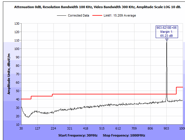
Plot 11. Radiated Spurious Emissions, 902.3 MHz, 30 – 1000 MHz
