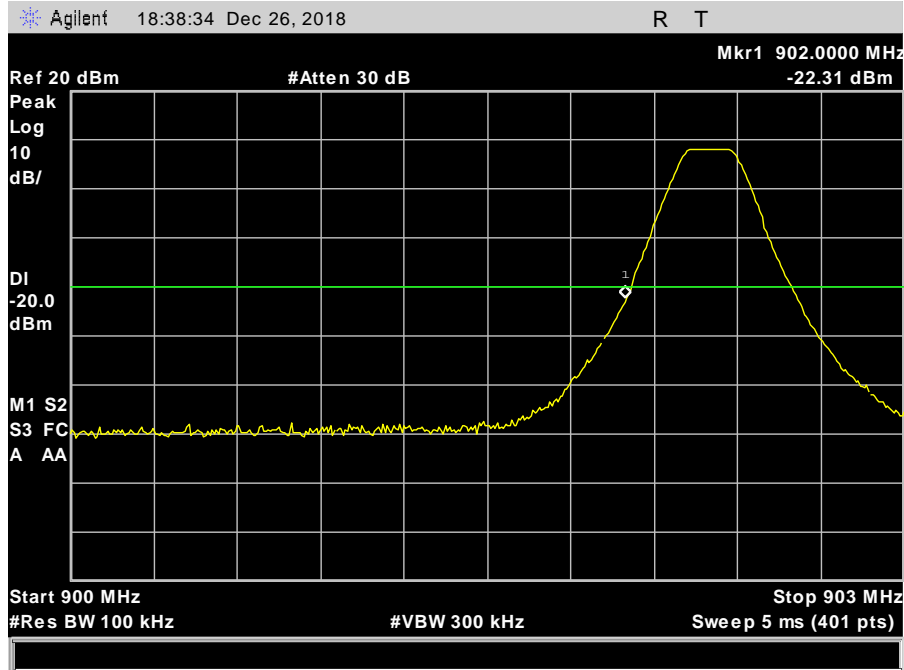
Plot 25. Conducted Band Edge, 902.3 MHz
