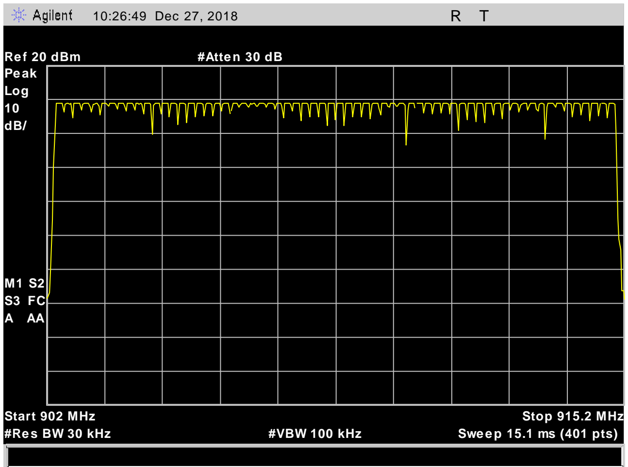
Plot 6. Number of Channels, 64 Channels
