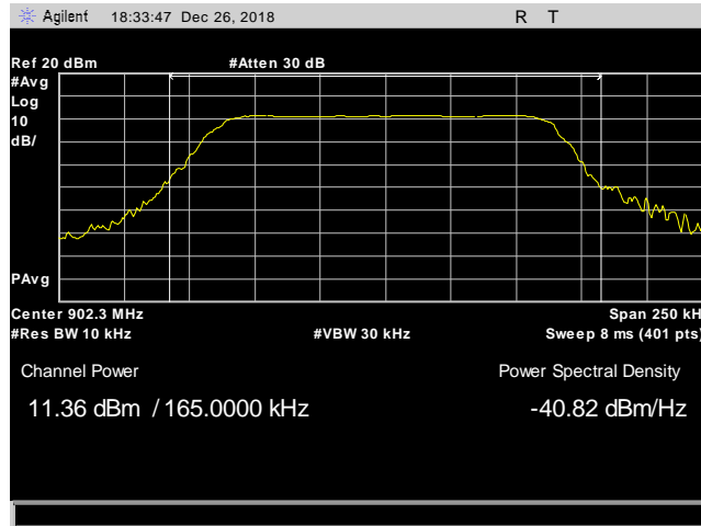
Plot 8. Power Output, 902.3 MHz, 11.36 dBm
