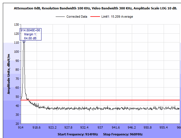
Plot 21. Radiated Restricted Band Edge, 914.9 MHz
