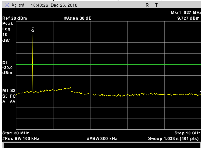
Plot 24. Conducted Spurious Emissions, 914.9 MHz, 30 MHz – 10 GHz
