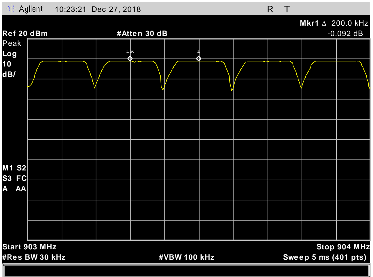
Plot 7. Channel Separation, 200 kHz
