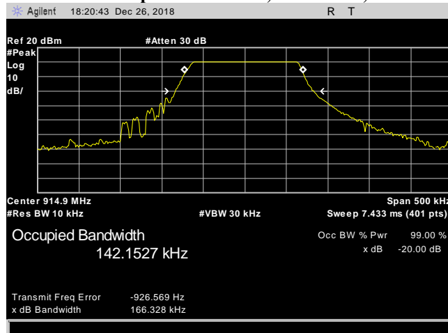
Plot 3. 20 dB Occupied Bandwidth, 914.9 MHz, 166.328 kHz
