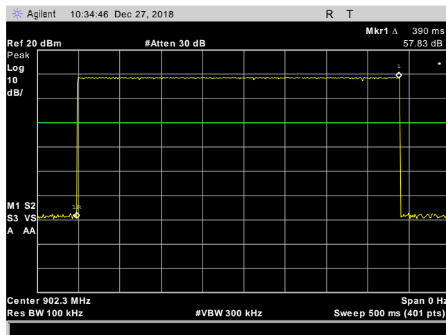
Plot 5. Dwell Time, Single Pulse
