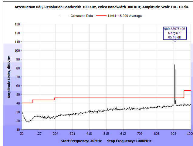
Plot 14. Radiated Spurious Emissions, 908.7 MHz, 30 – 1000 MHz
