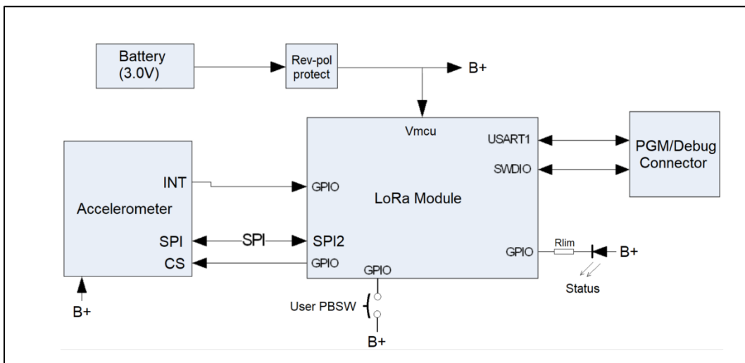
Figure 1. Asset Tracker: model: CR123 Block Diagram containing LoRa Module
