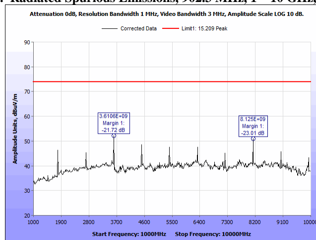
Plot 13. Radiated Spurious Emissions, 902.3 MHz, 1 – 10 GHz, Peak
