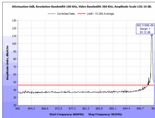
Plot 20. Radiated Restricted Band Edge, 902.3 MHz
