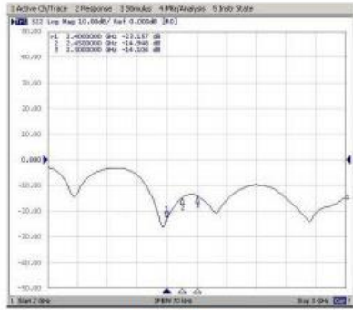
Return Loss
