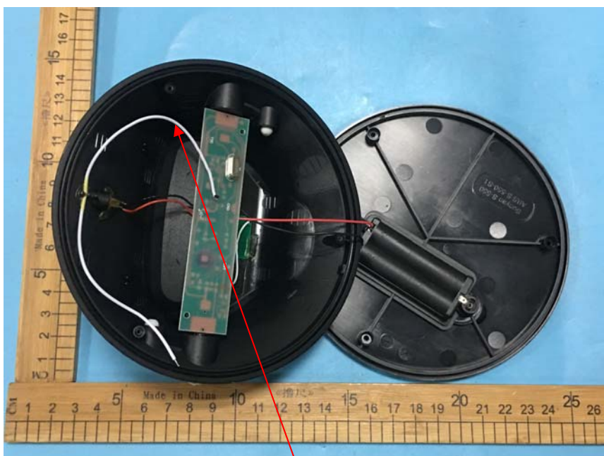
Wire Antenna
