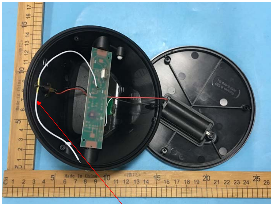
Wire Antenna
