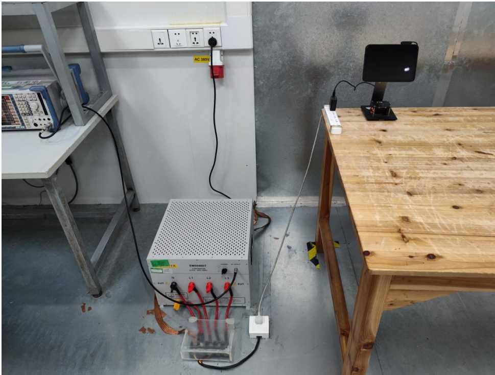
FCC ID: 2ARI5-MCST1-01 Photo of Conducted Emission Measurement
