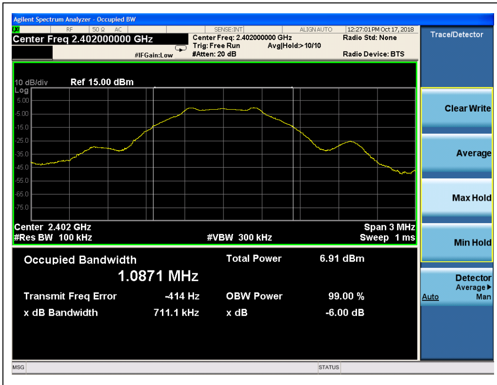
(Channel 0, 2402MHz)
