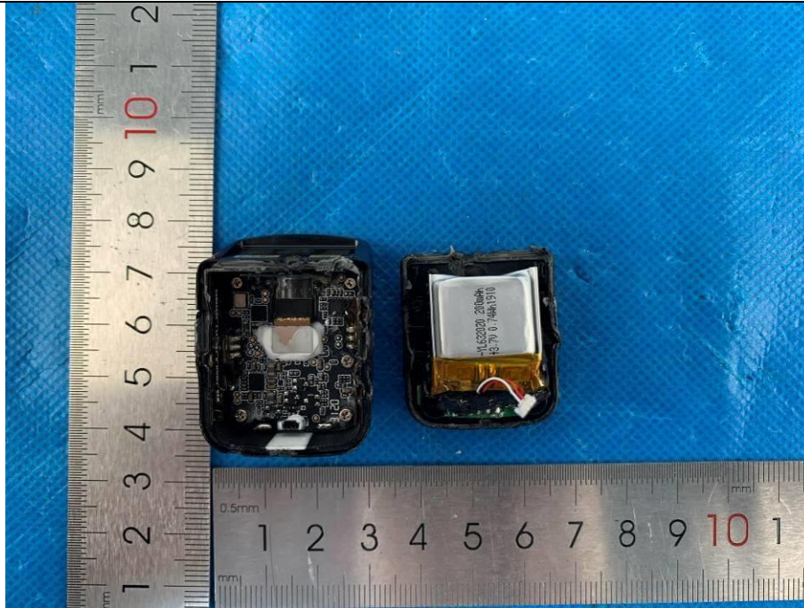
Photo 1 (For model W28)
