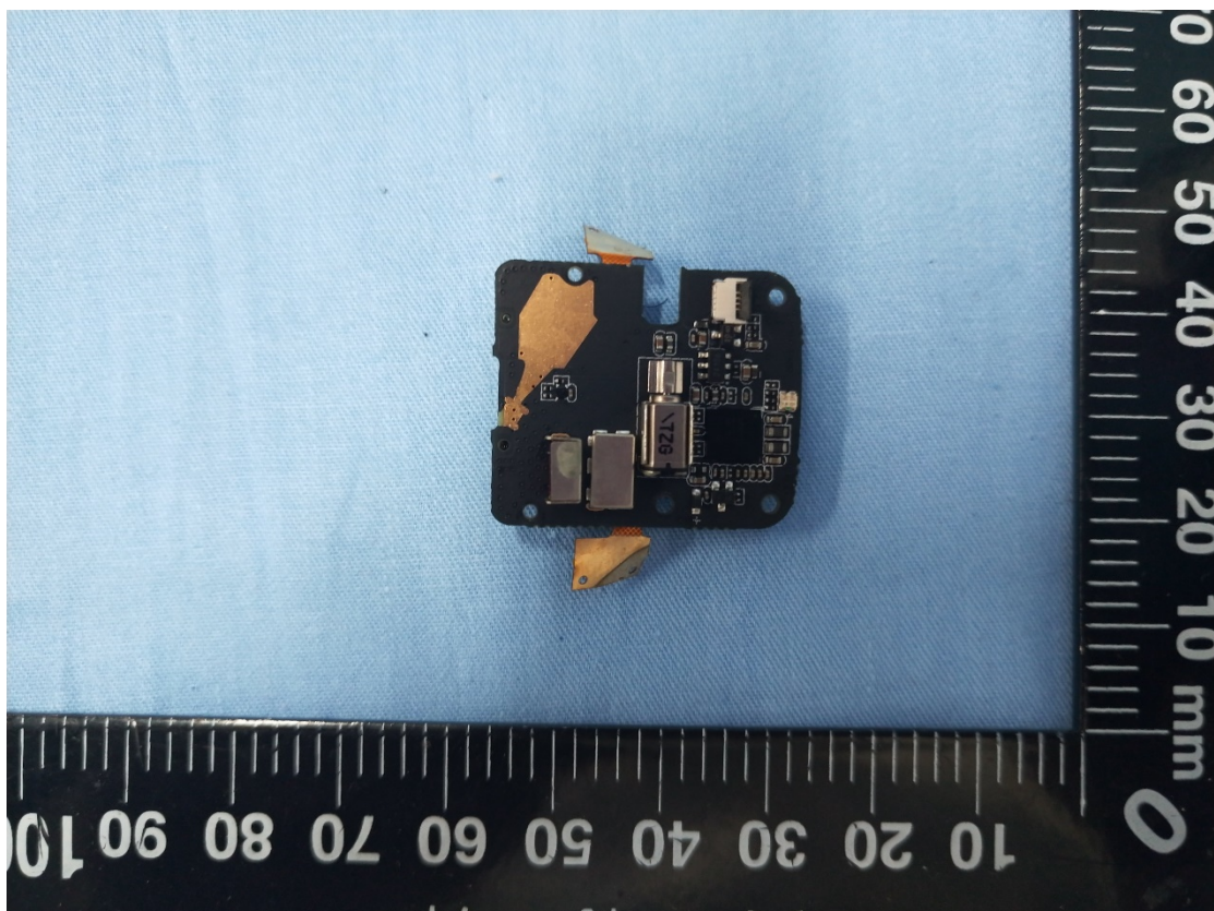
6. main board bottom view
