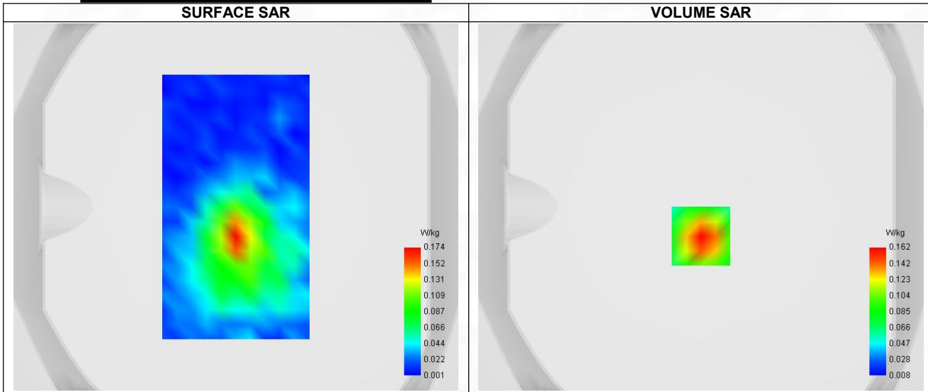
Maximum location: X=0.00, Y=-16.00 ; SAR Peak: 0.26 W/kg
