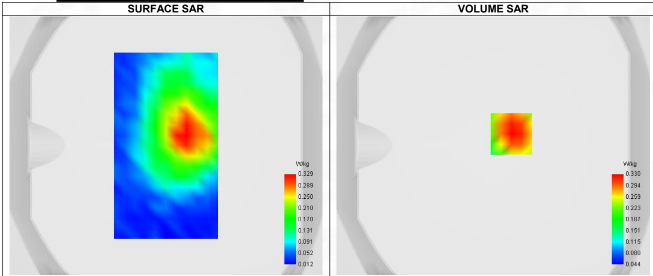
Maximum location: X=14.00, Y=9.00 ; SAR Peak: 0.45 W/kg
