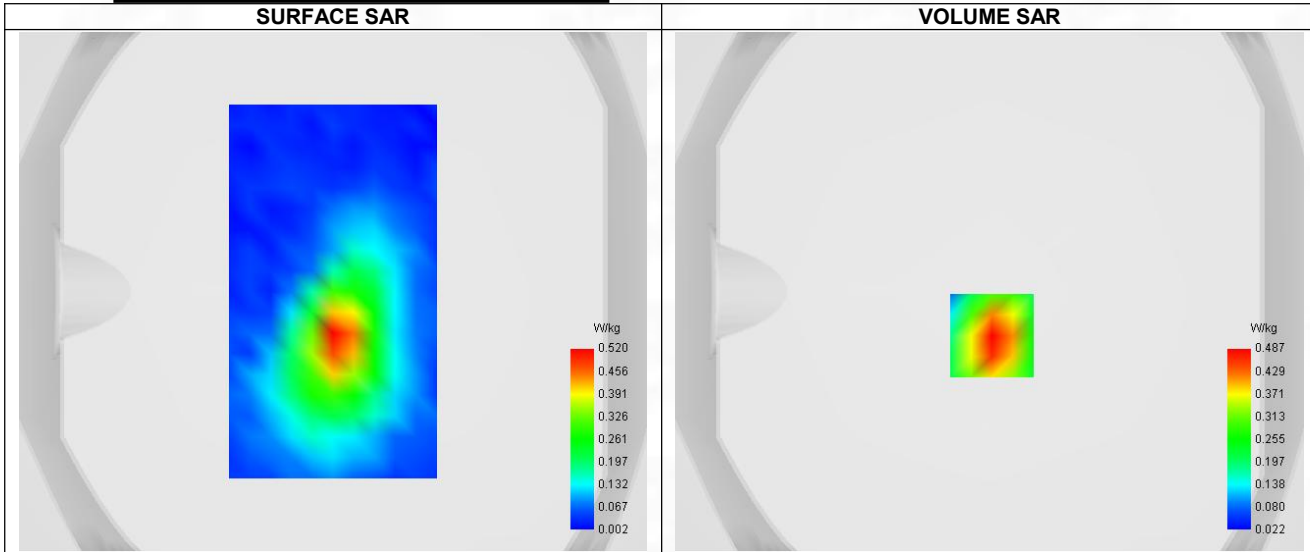
Maximum location: X=5.00, Y=7.00 ; SAR Peak: 0.72 W/kg
