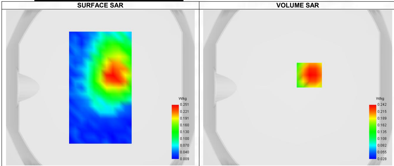
Maximum location: X=15.00, Y=16.00 ; SAR Peak: 0.33 W/kg
