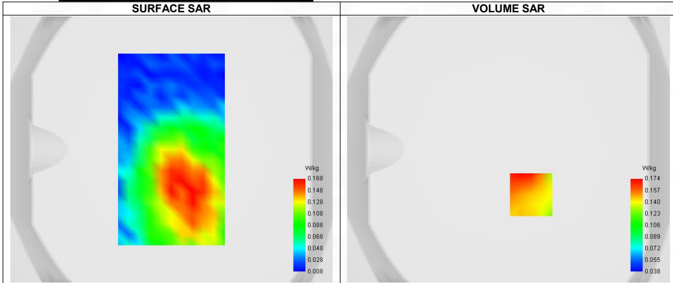
Maximum location: X=17.00, Y=-34.00 ; SAR Peak: 0.25 W/kg
