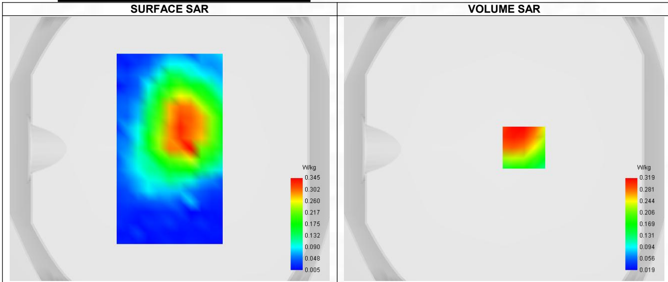
Maximum location: X=15.00, Y=1.00 ; SAR Peak: 1.30 W/kg
