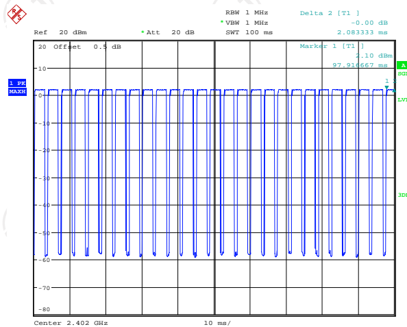
3DH5 on time (Count Pulses) Plot on Channel 00
