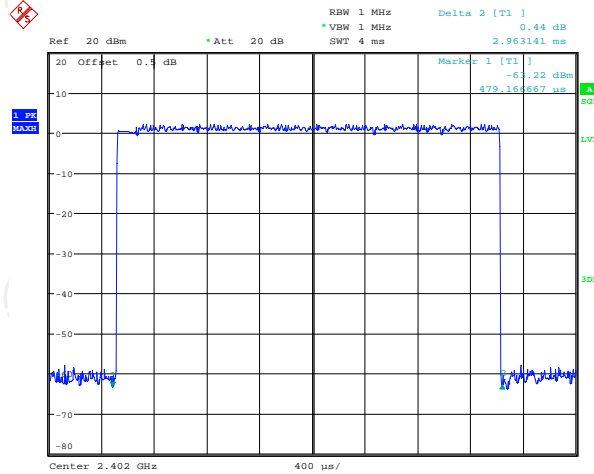
3DH5 on time (One Pulse) Plot on Channel 00
