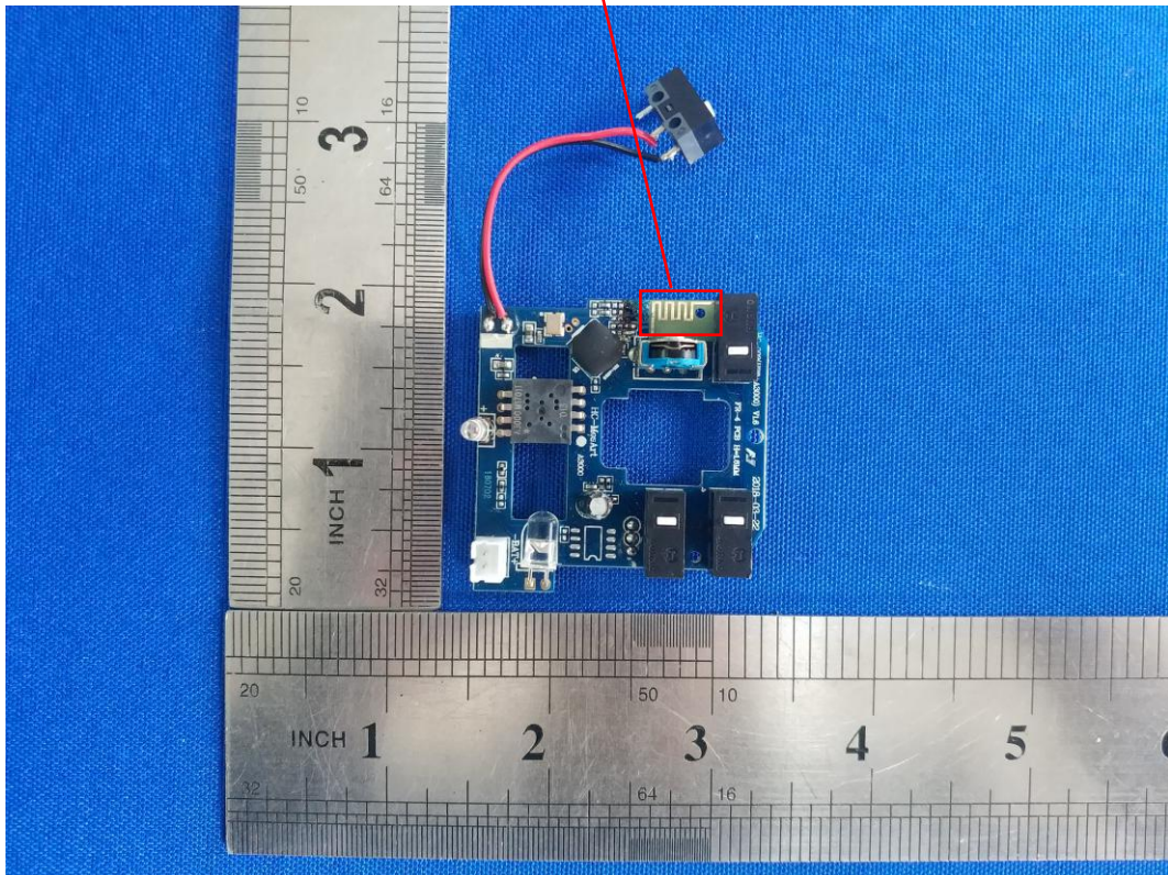
PCB antenna
