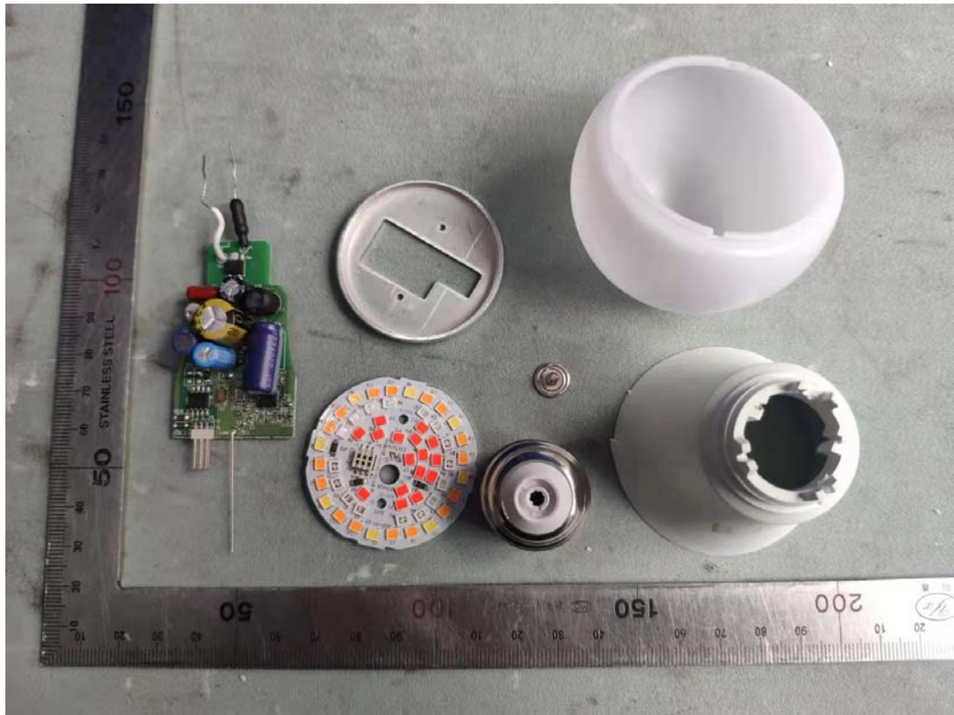
FIGURE 1 ABODE COLOR BULB (M/N: 104062/A) GENERAL APPEARANCE (COVER REMOVED)
