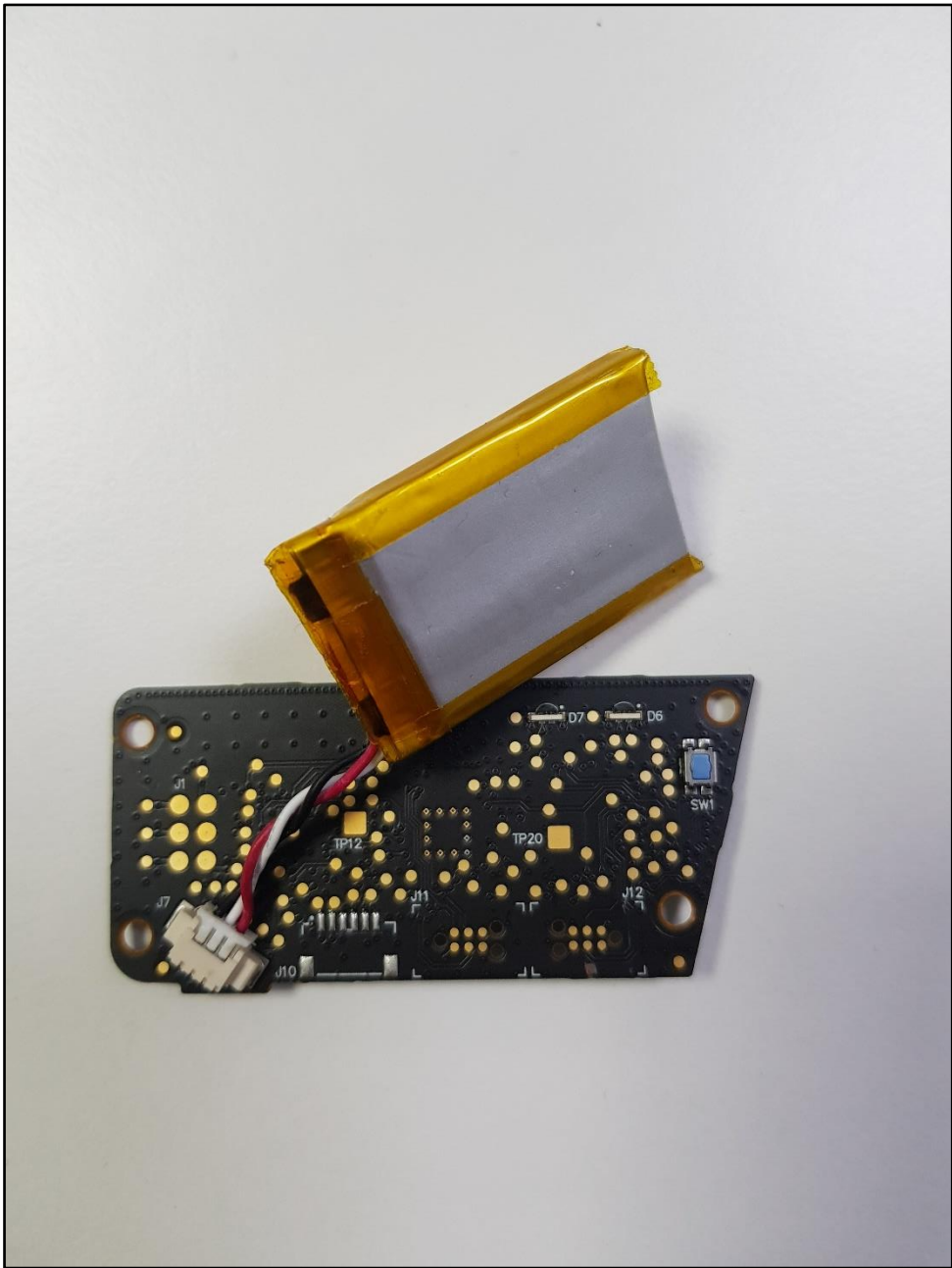
Figure 6: Right Tracker Internal – Back with Battery
