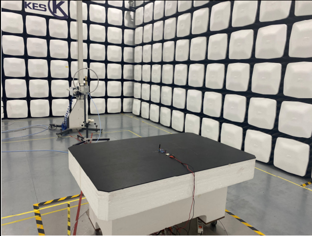
Radiated emissions
