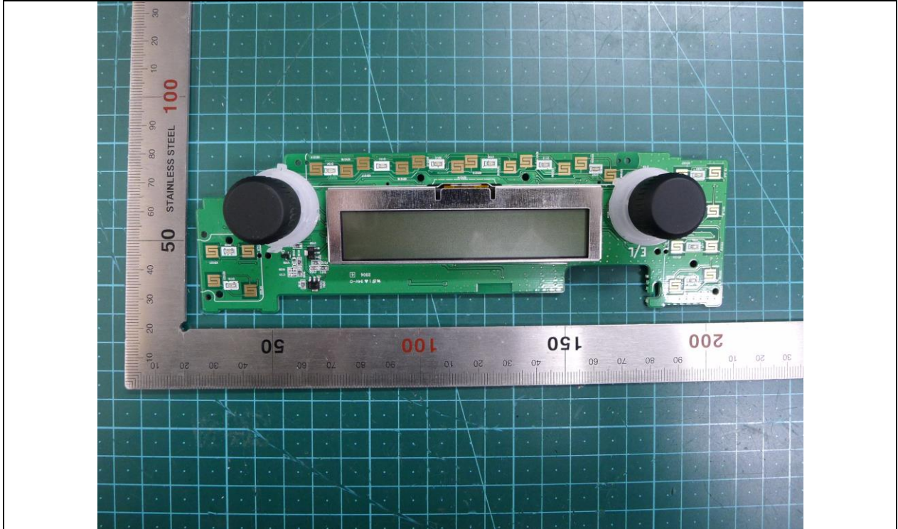
Front PCB Front
