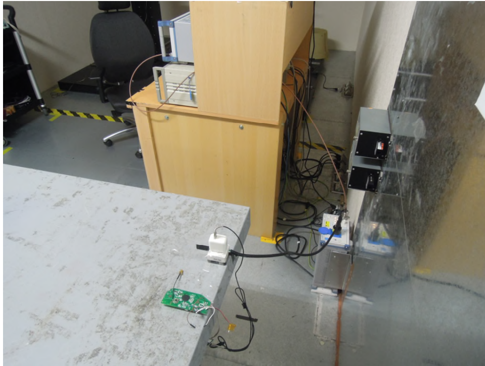
Photograph 11: Set-up for Mains Conducted testing
