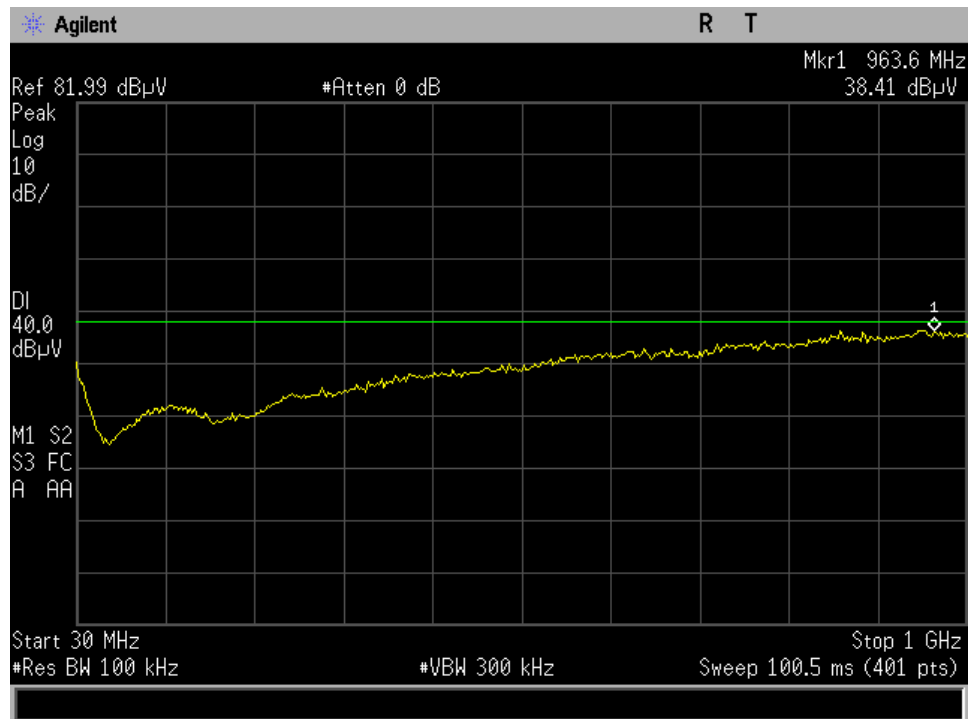
30MHz-1GHz Mid channel Restricted Band
