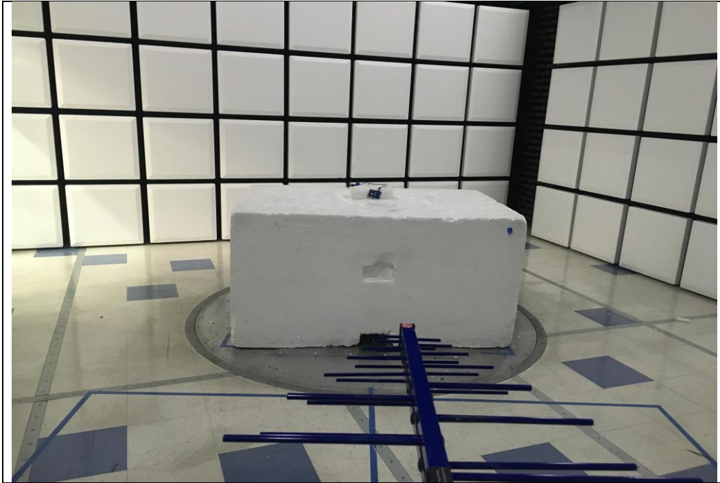
RF Radiated #2
