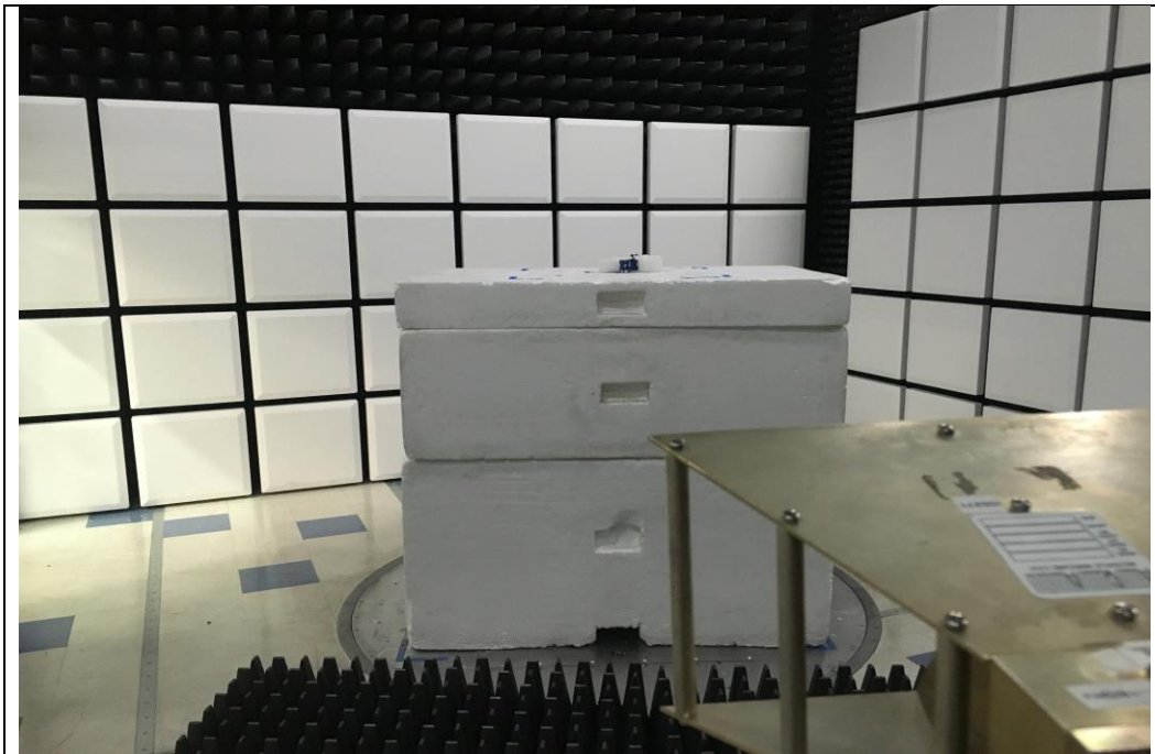
RF Radiated #2
